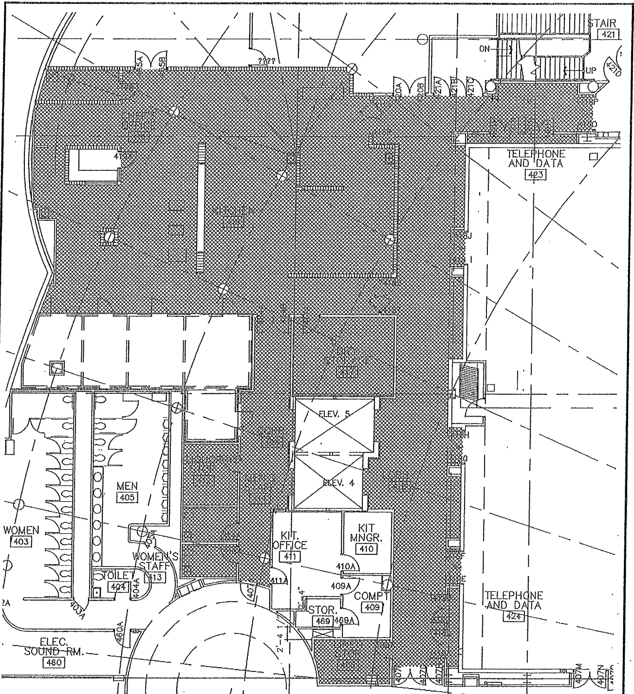
1 ENLARGED LEVEL +40' FLOOR PLAN 1/16" = 1'-0"
