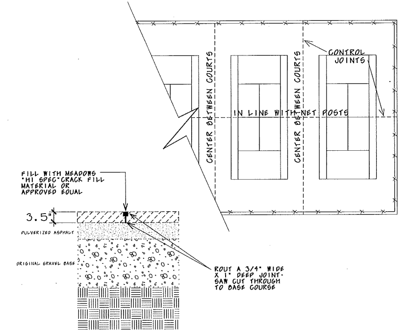
TENNIS COURT CONTROL JOINTS DETAIL 2 NO SCALE
