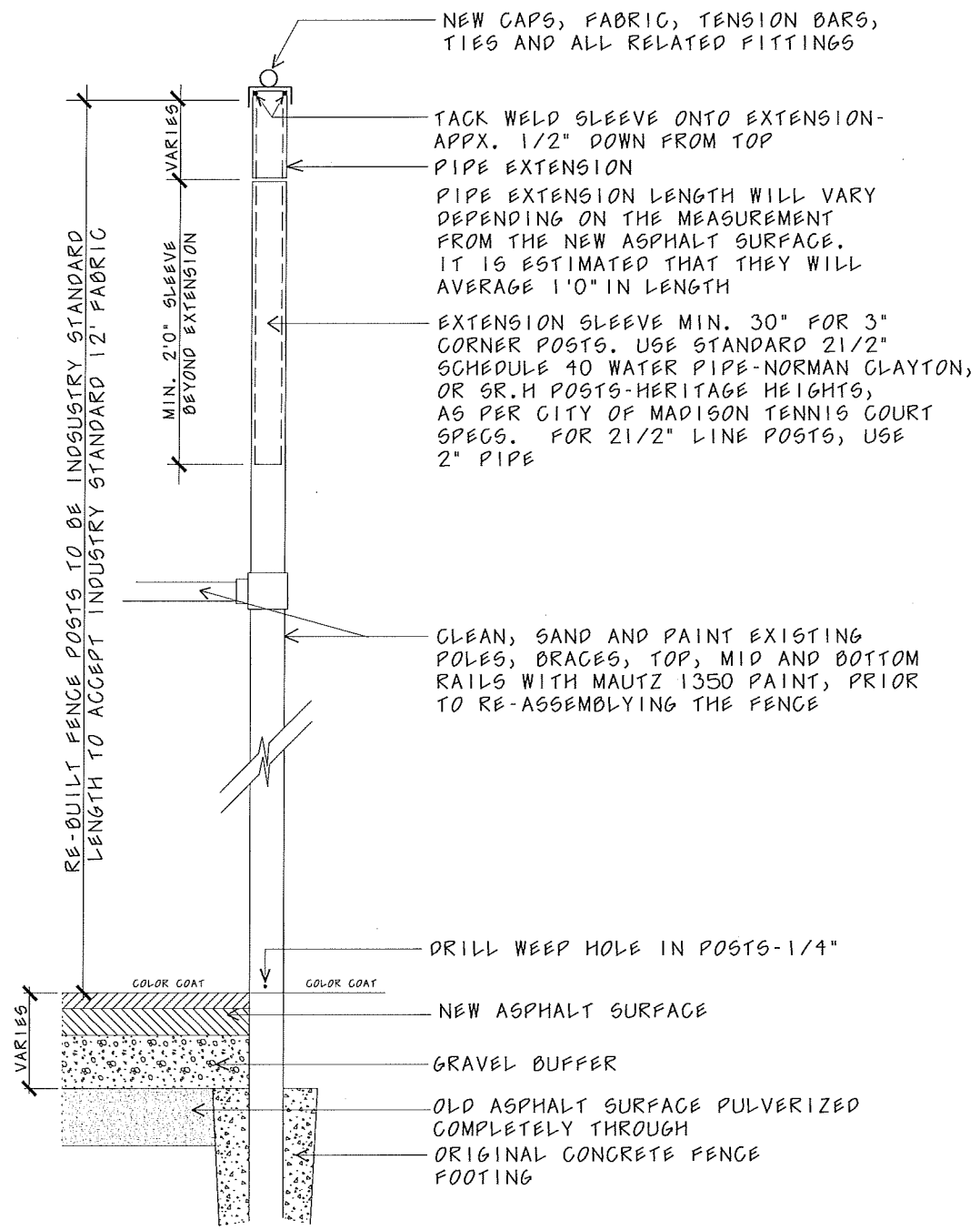
TENNIS COURT FENCE EXTENSION AND REPAIR DETAIL 1
