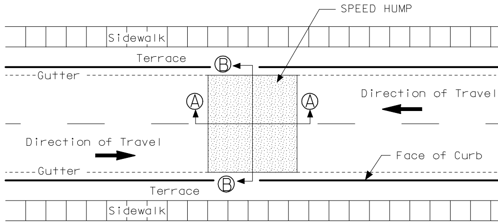
SPEED HUMP ON TYPICAL URBAN STREET
