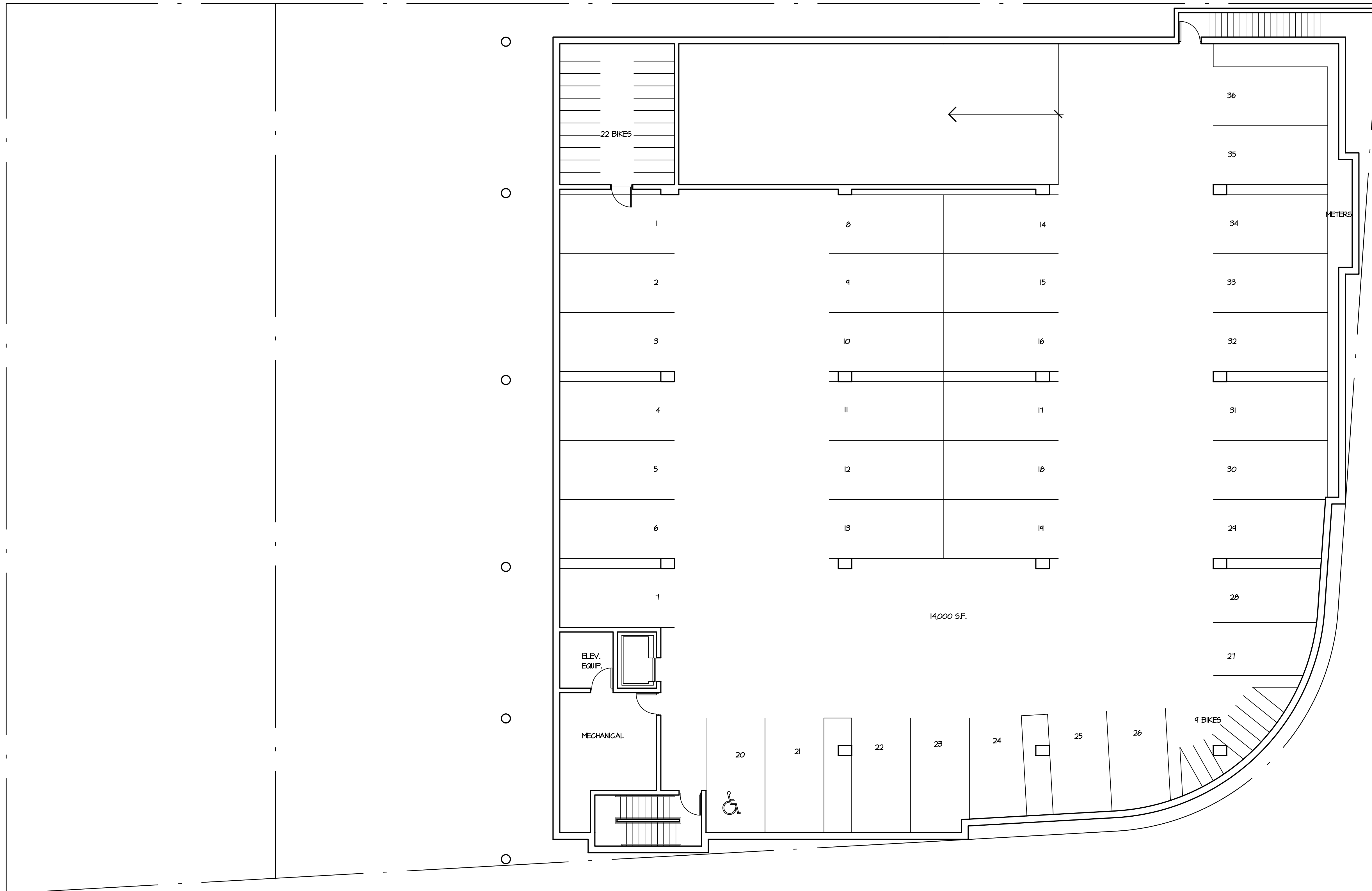
1 A1 PARKING LEVEL PLAN - SCHEME B SCALE 1/8" = 1'-0"
