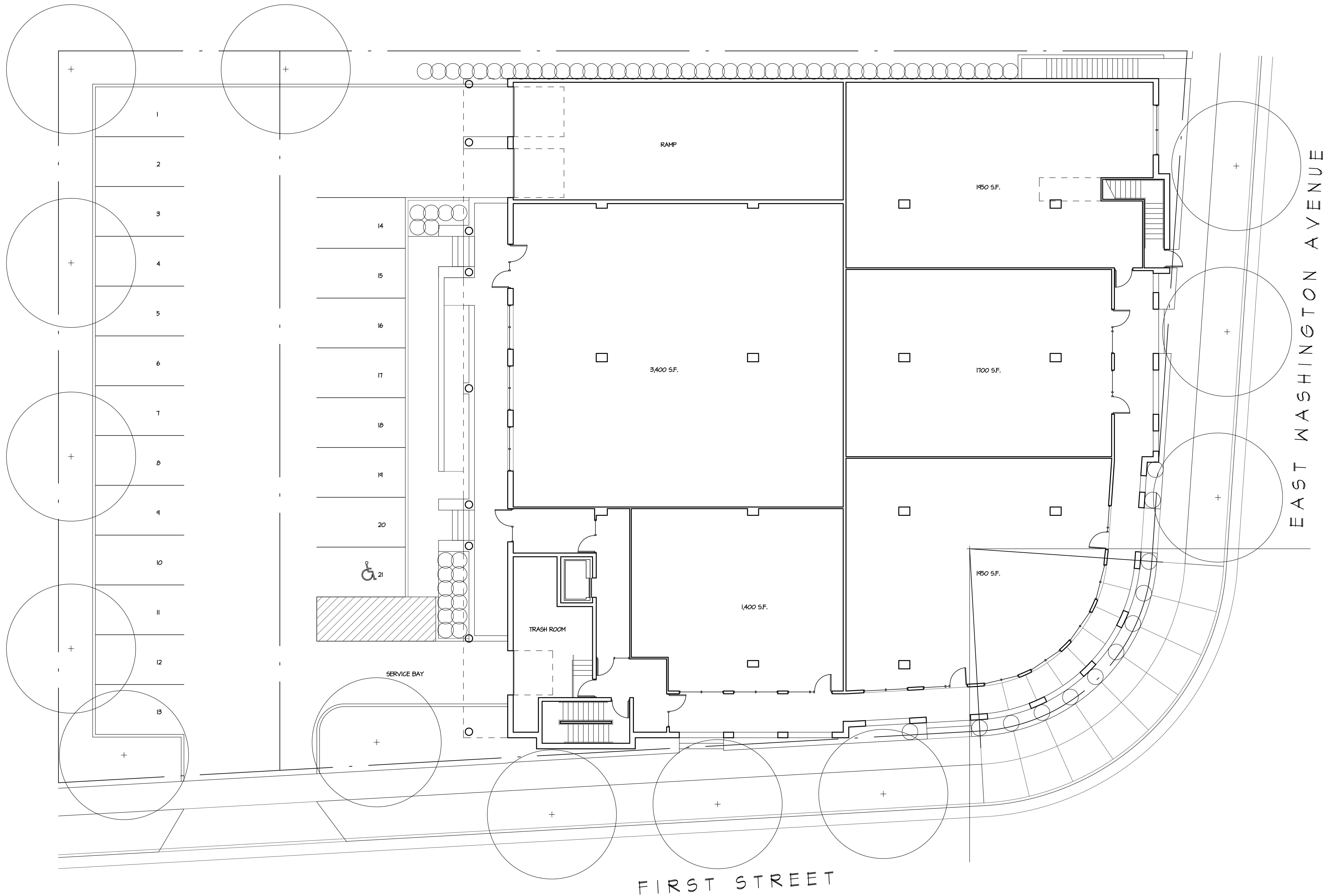
1 SITE/FIRST FLOOR PLAN - SCHEME B A2 SCALE 1/8" = 1'-0"
