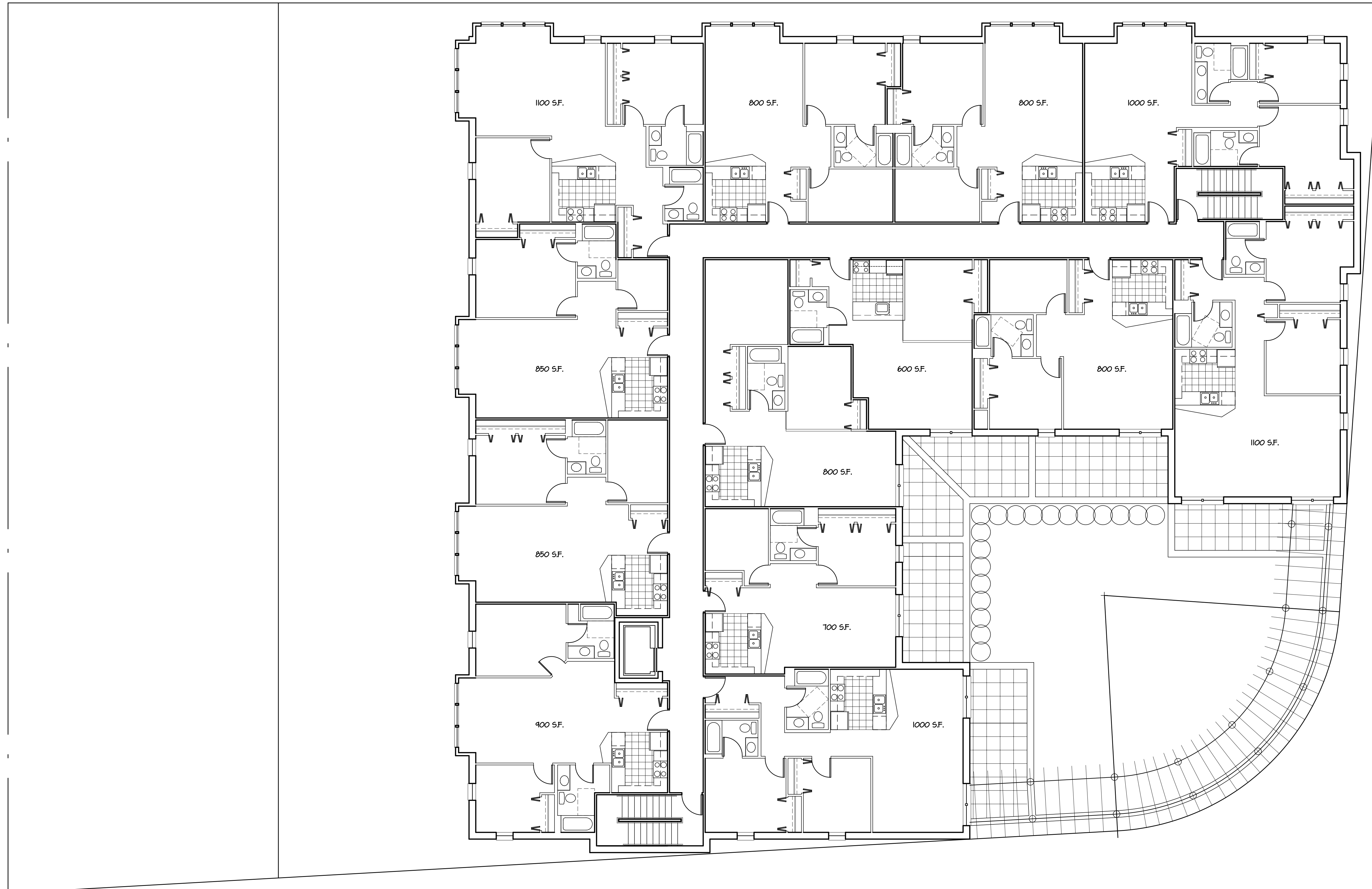
TYPICAL FLOOR PLAN - SCHEME B SCALE 1/8" = 1'-0"
