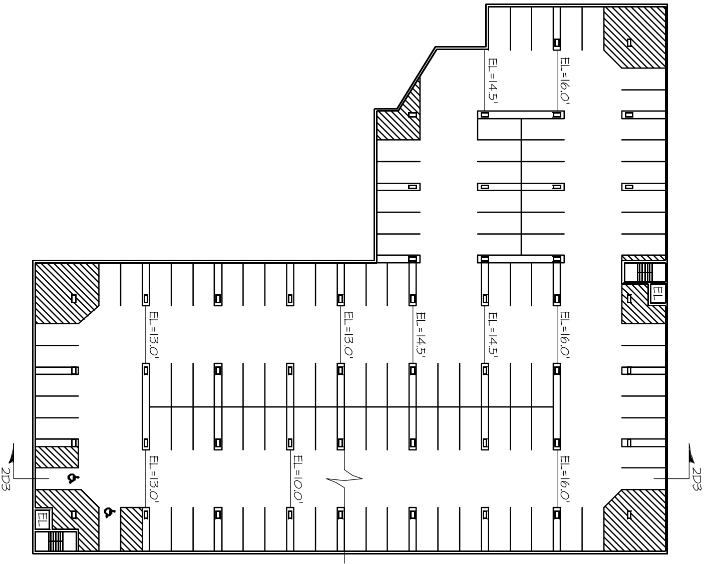
LEVEL L2
