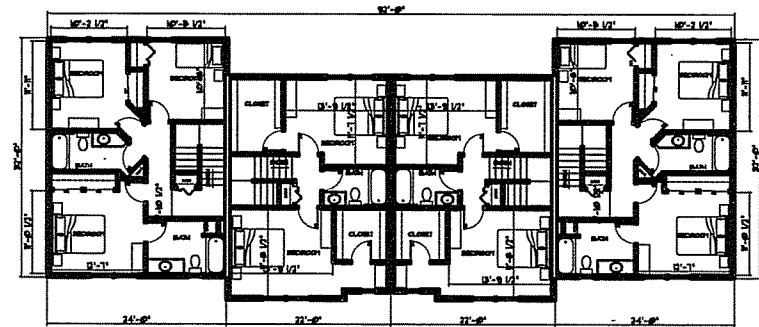
PROPOSED SECOND FLOOR SCALE 1/8" = 1'-0"
