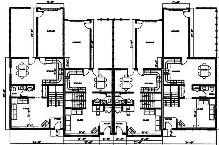
PROPOSED FIRST FLOOR SCALE 1/8" = 1'-0"
