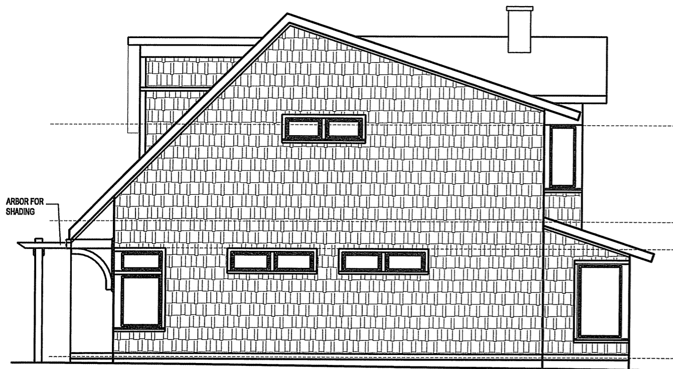
3 EAST ELEVATION 1/8" = 1'-0"
