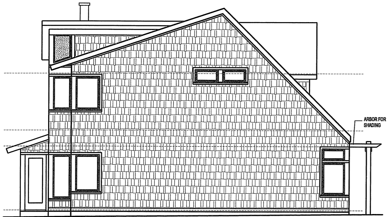
4 WEST ELEVATION 1/8" = 1'-0"
