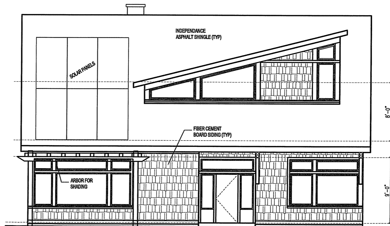
1 FRONT ELEVATION 1/8" = 1'-0"
