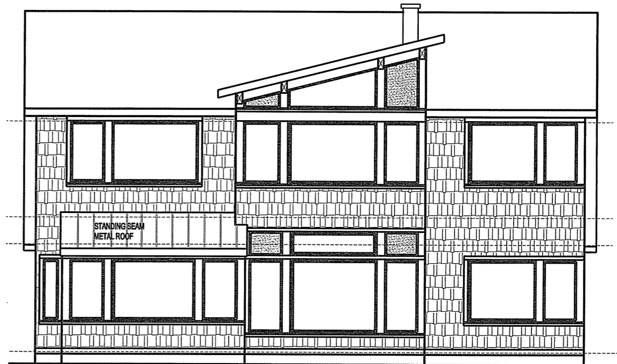
2 LAKEFRONT ELEVATION 1/8" = 1'-0"
