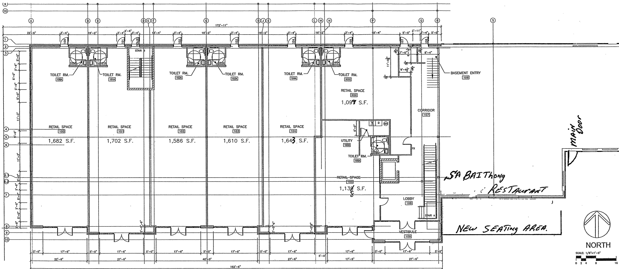
1 FIRST FLOOR PLAN 0 2 4 8 16 FEET
