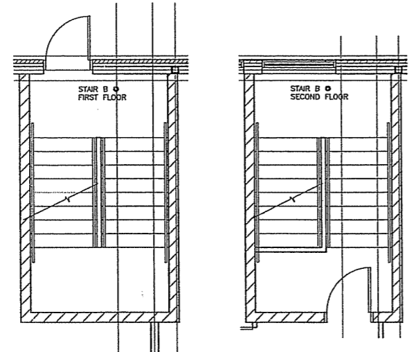
3 STAIR B PLAN 1/4"=1'-0"
