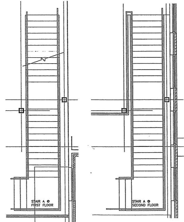
4 STAIR A PLAN 1/4"=1'-0"
