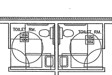
2 FIRST FLOOR TOILET ROOMS 1/4"=1'-0"
