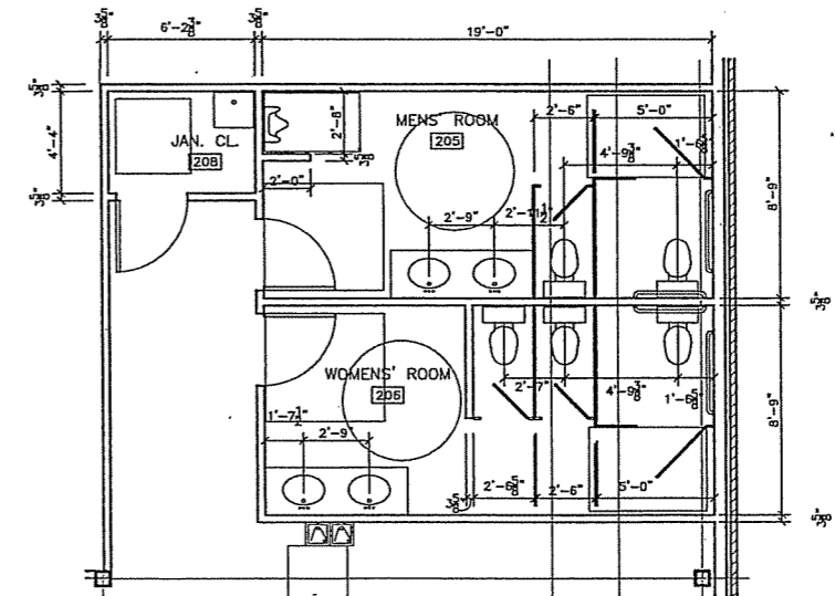
5 SECOND FLOOR TOILET ROOMS 1/4"=1'-0"
