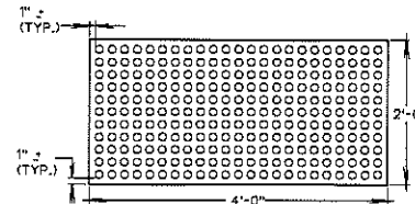
PLAN VIEW DETECTABLE WARNING FIELD (TYPICAL)
