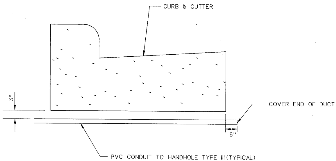
LOOP LEAD DUCT DETAIL
