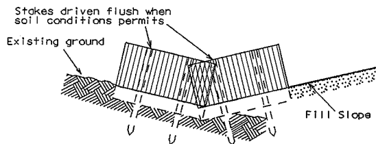
FRONT ELEVATION
