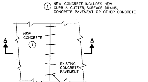
PLAN VIEW
