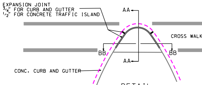
DETAIL CONCRETE TRAFFIC ISLAND CROSS WALK THRU ISLAND NOSE
