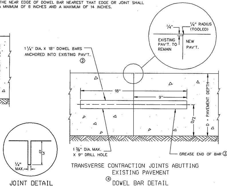
PAVEMENT DEPTH, DOWEL BAR SIZE AND JOINT SPACING TABLE
