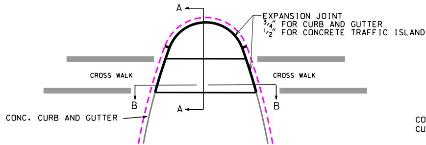
DETAIL CONCRETE TRAFFIC ISLAND CROSS WALK 2' OR FARTHER FROM END OF ISLAND NOSE
