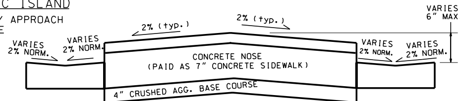
SECTION BBB-BBB
