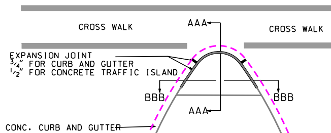
DETAIL CONCRETE TRAFFIC ISLAND CROSS WALK AT END / APPROACH ISLAND NOSE
