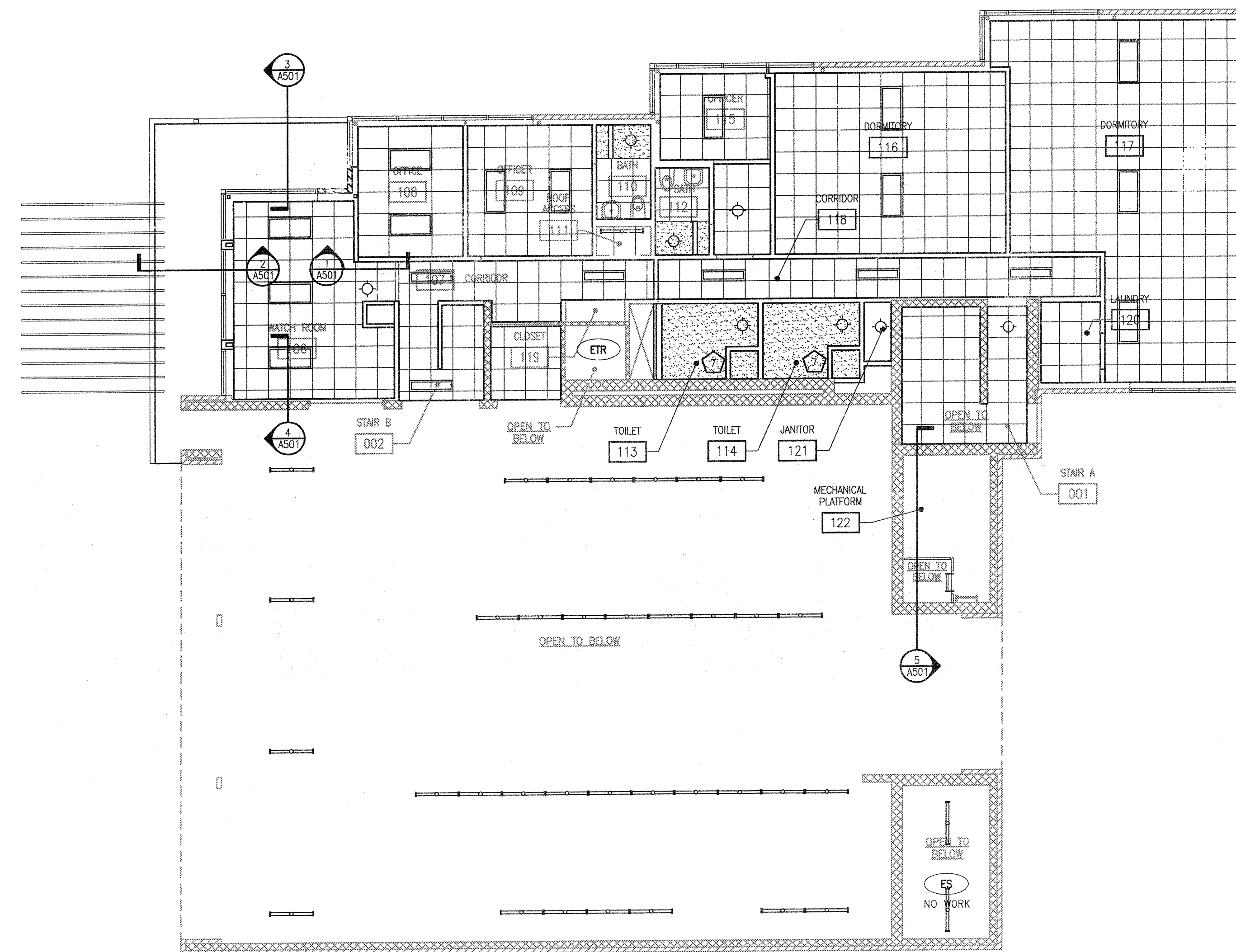
2 A301 UPPER LEVEL REFLECTED CEILING PLAN SCALE: 1/8" = 1'-0"
