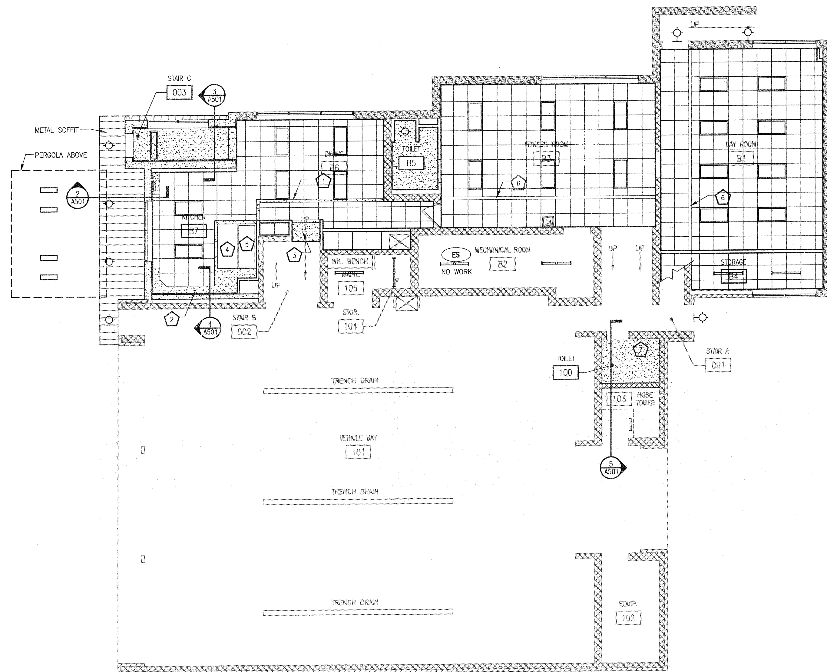
1 A301 LOWER LEVEL REFLECTED CEILING PLAN SCALE: 1/8" = 1'-0"
