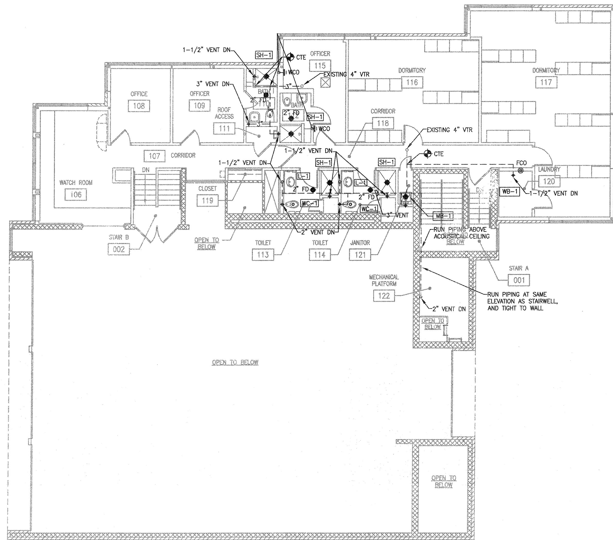
UPPER LEVEL WASTE ADDITION AND REMODELING PLAN SCALE: 1/8" = 1'-0"
