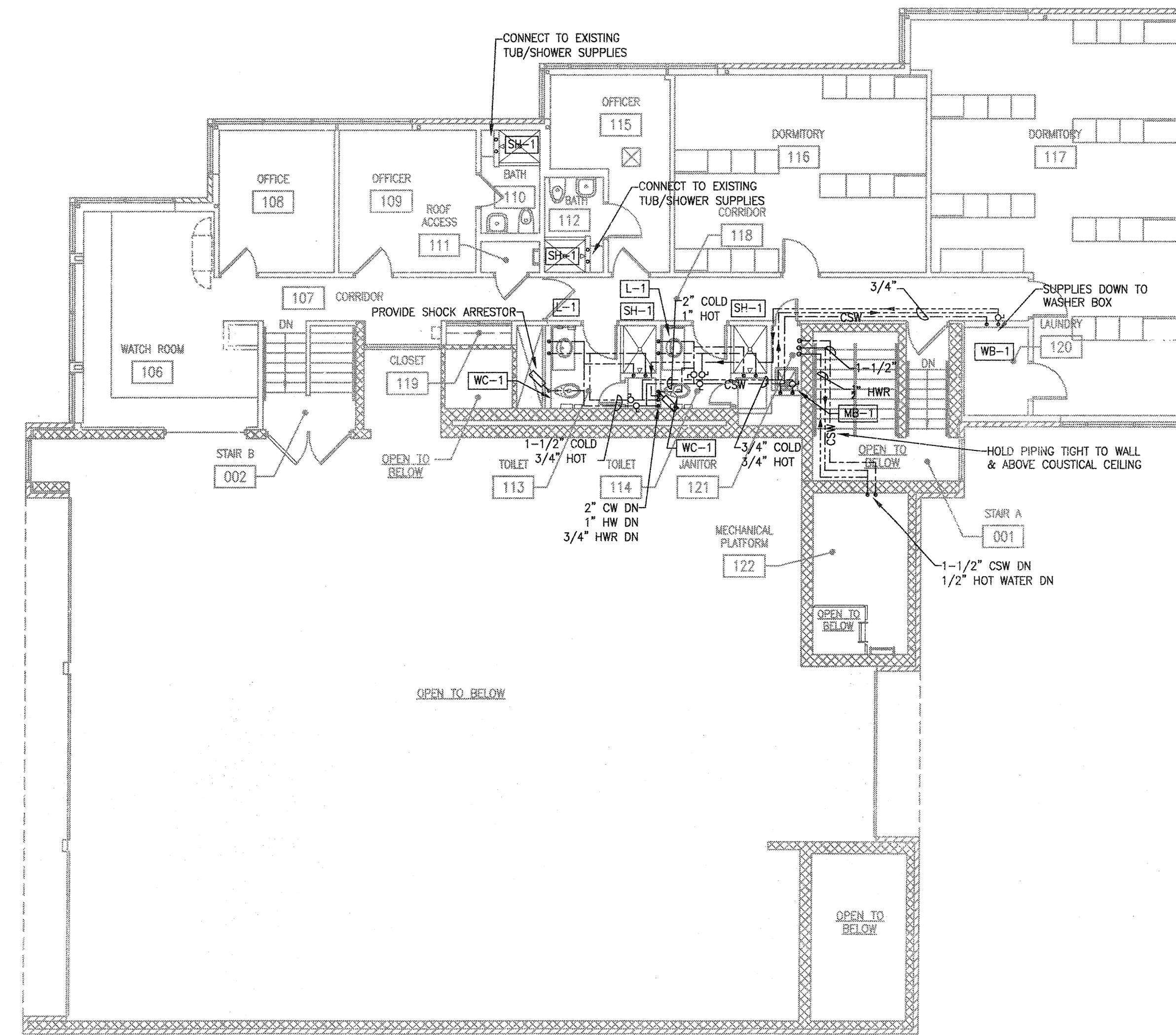
UPPER LEVEL SUPPLY ADDITION AND REMODELING PLAN SCALE: 1/8" = 1'-0"
