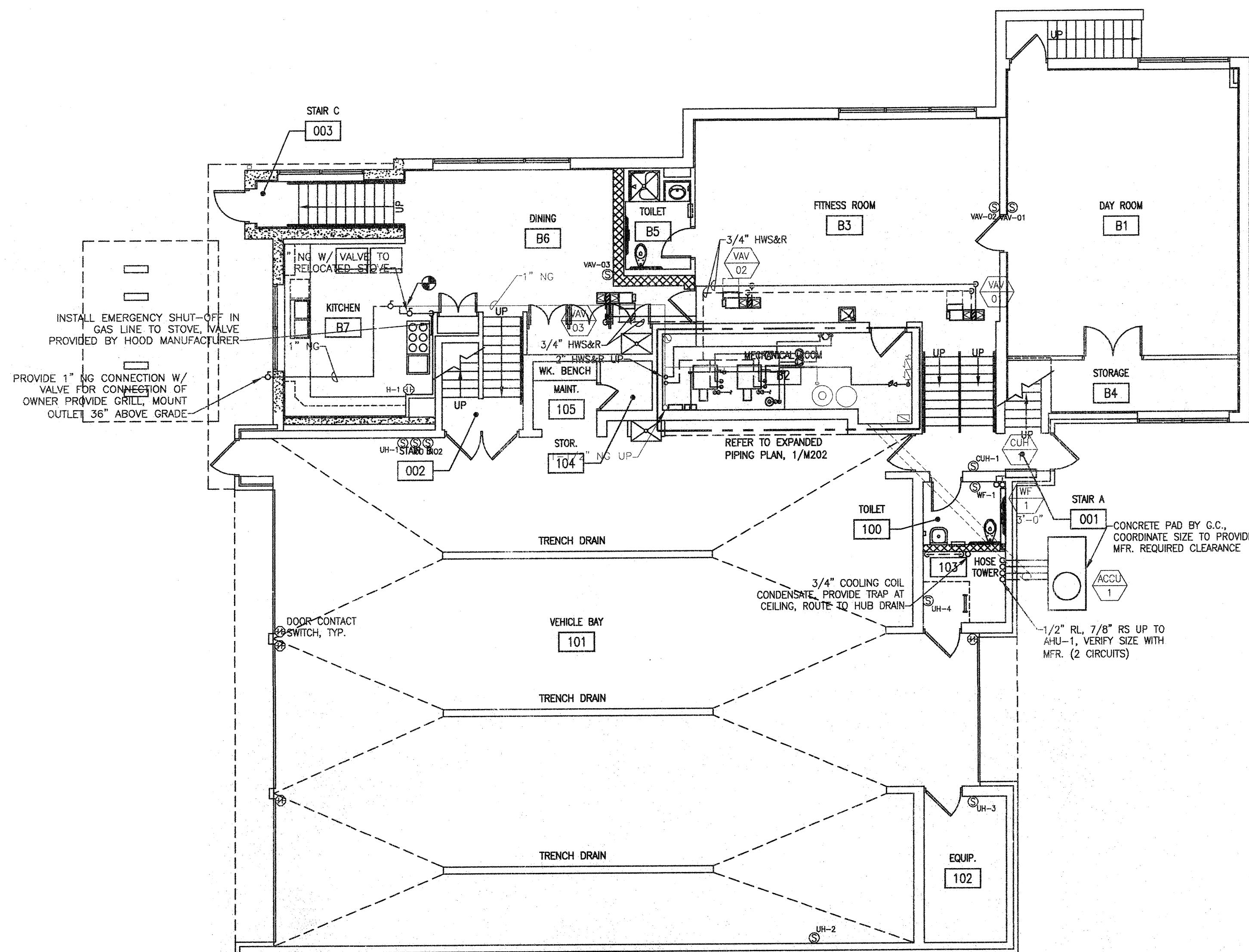
3 LOWER LEVEL HVAC PIPING PLAN SCALE: 1/8" = 1'-0"
