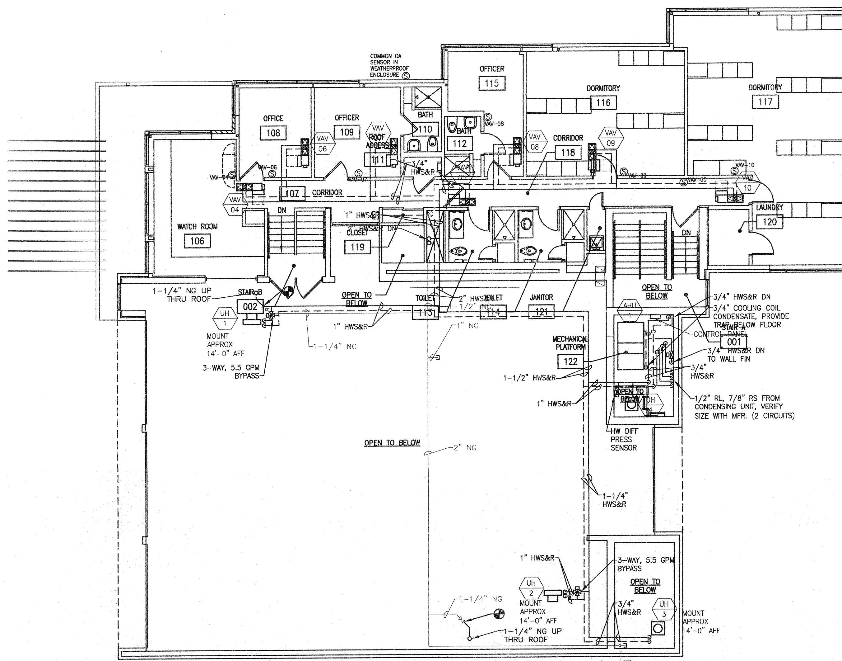
4 UPPER LEVEL HVAC PIPING PLAN SCALE: 1/8" = 1'-0"
