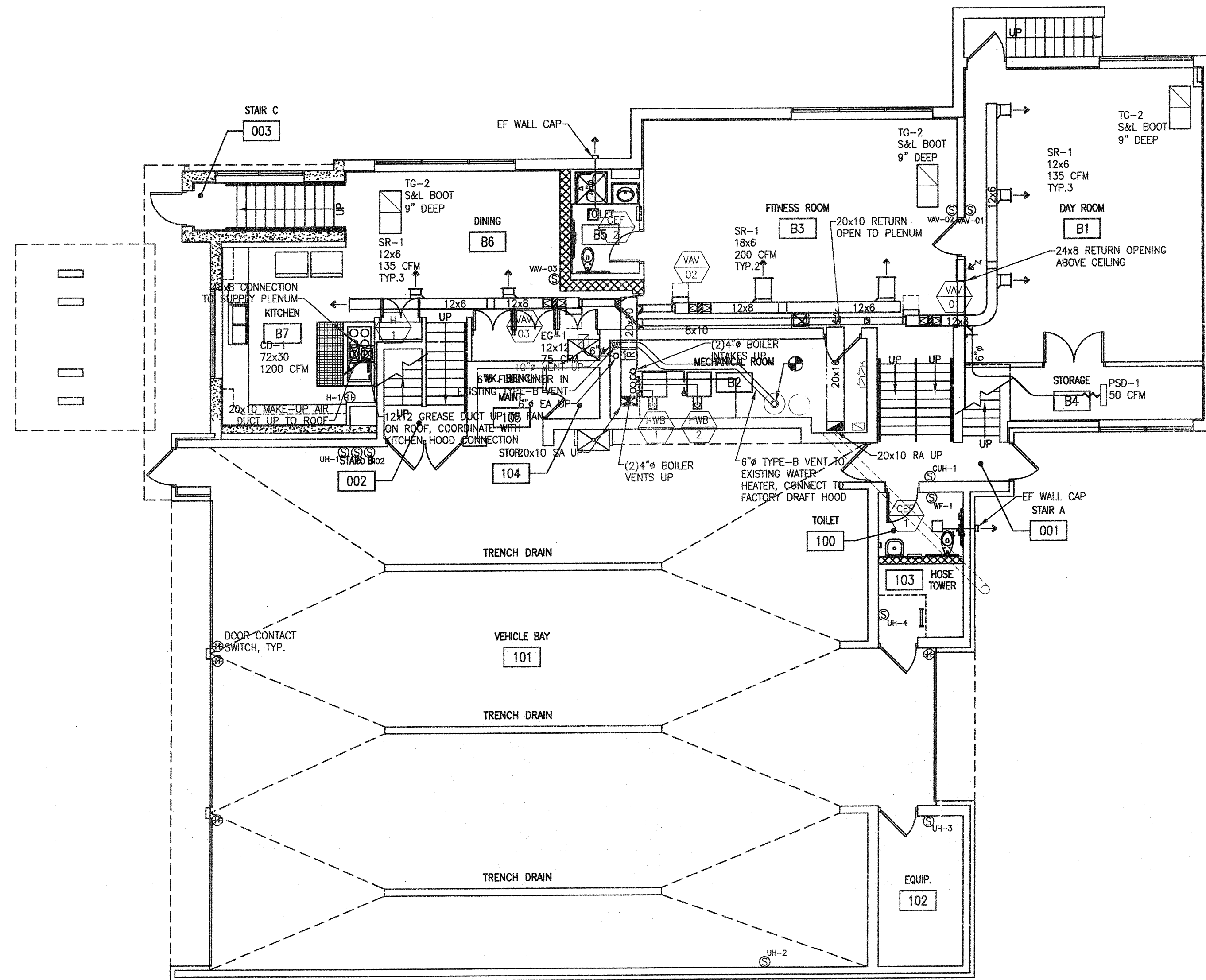
1 LOWER LEVEL HVAC REMODELING PLAN SCALE: 1/8" = 1'-0"
