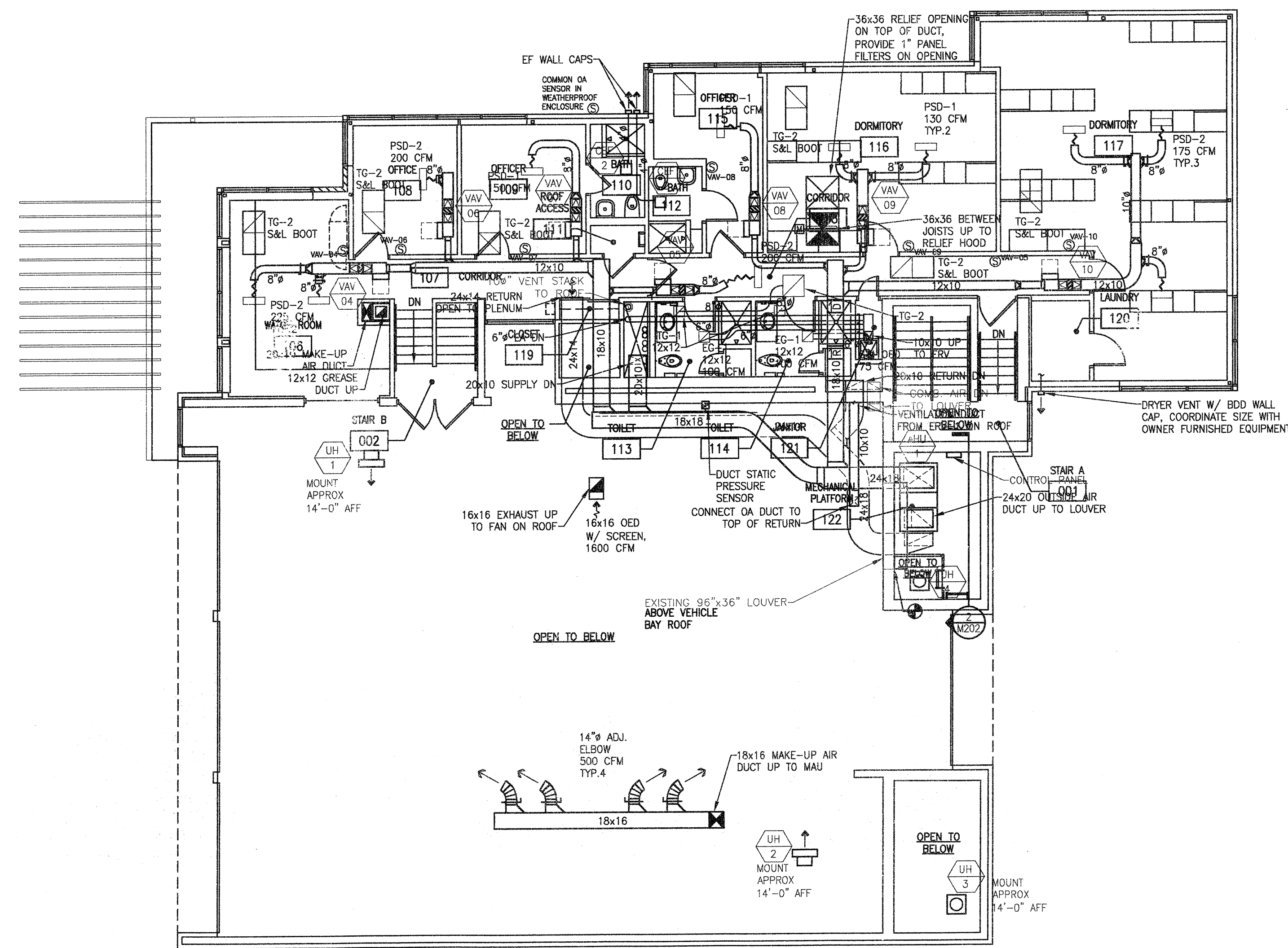
2 UPPER LEVEL HVAC REMODELING PLAN SCALE: 1/8" = 1'-0"
