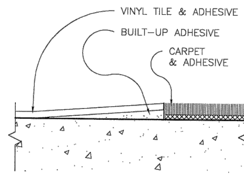
4 - Vinyl to Carpet (no scale)
