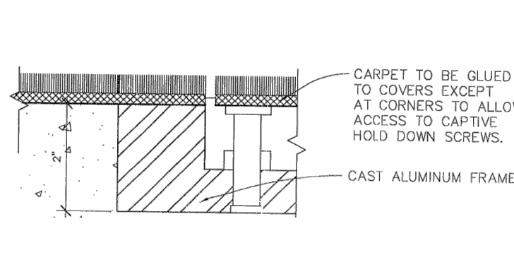
5 - Floor Box w/Carpet (no scale)
