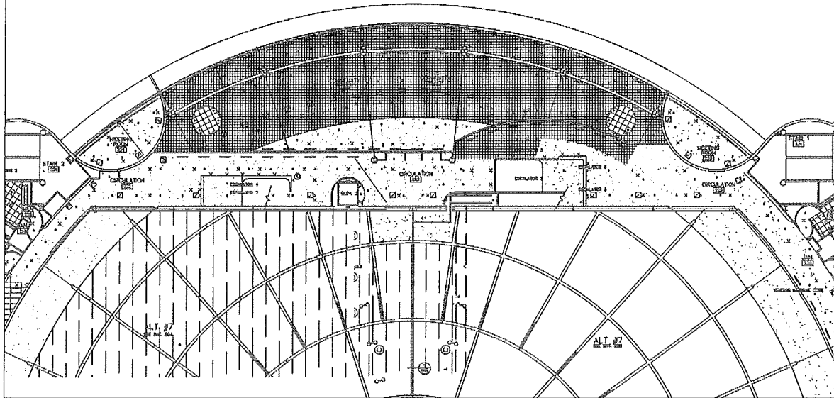
1 ENLARGED LEVEL +19' CEILING PLAN 1/16" = 1'-0"
