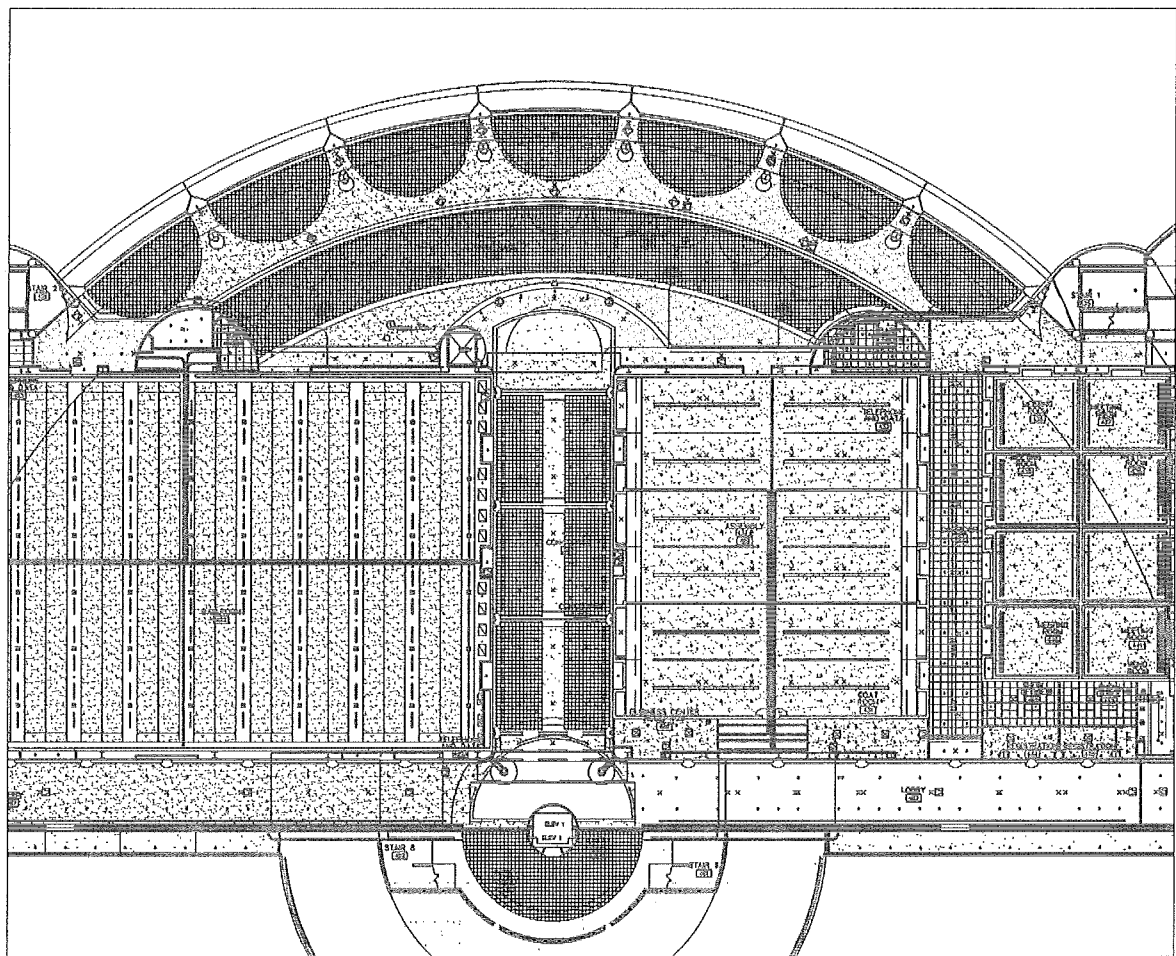
2 ENLARGED LEVEL +40' CEILING PLAN 1/16" = 1'-0"
