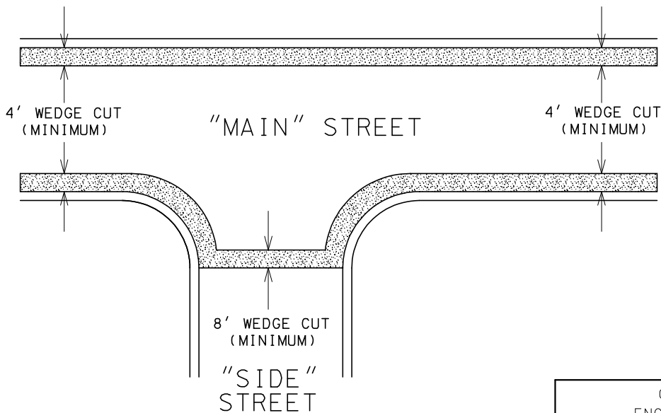
DETAIL "C" RADIUS RETURN CUTS
