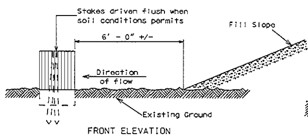
EROSION BALES AT TOE OF SLOPE WHEN EXISTING GROUND SLOPES AWAY FROM FILL SLOPE
