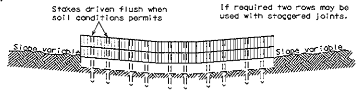
FRONT ELEVATION
