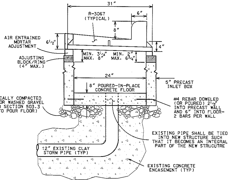
PRECAST OPTION
