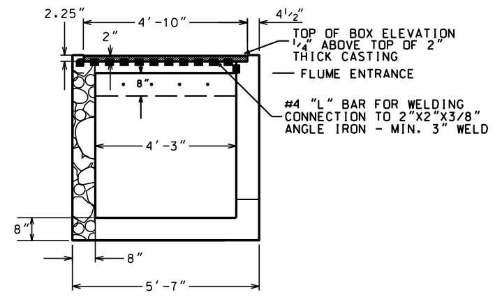
SECTION 1
