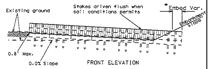
EROSION BALES AT TOE OF SLOPE
