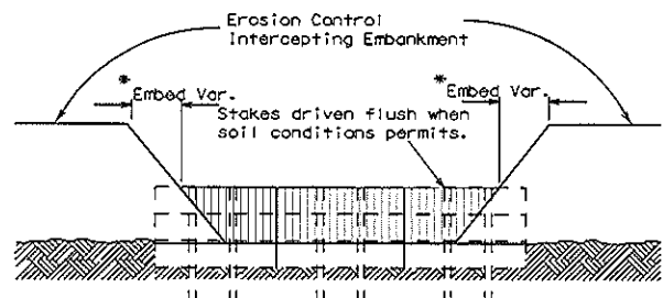
EROSION CONTROL INTERCEPTING EMBANKMENT
