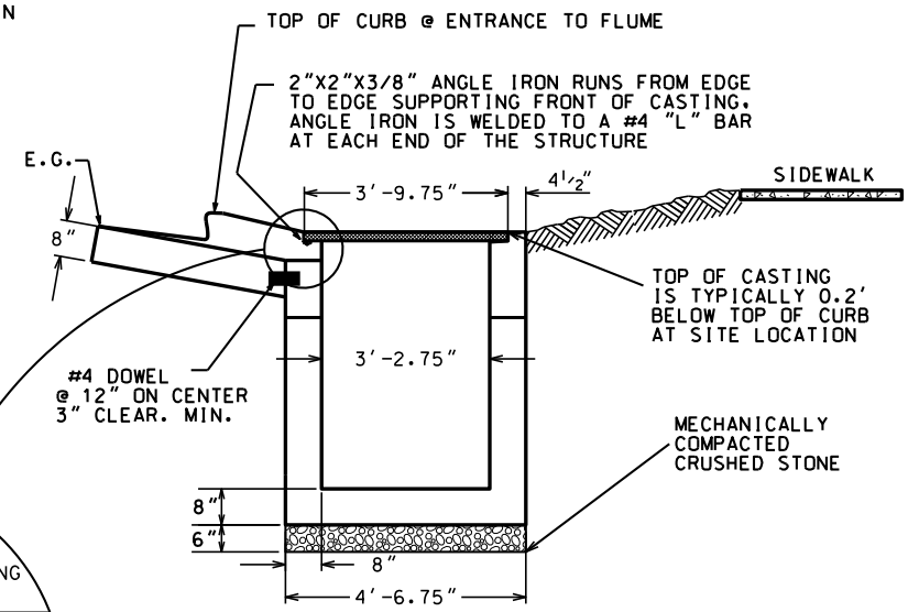
SECTION 2
