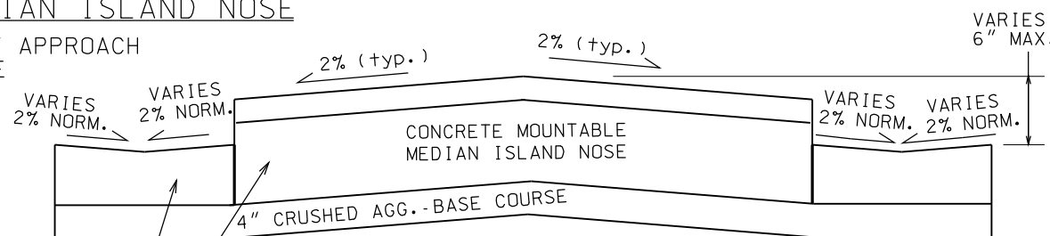
SECTION BBB-BBB
