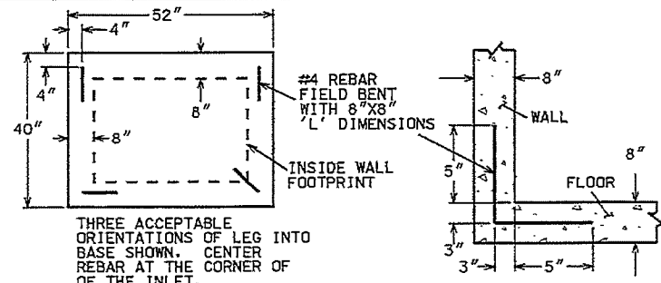
FIELD POURED FLOOR REINFORCEMENT
