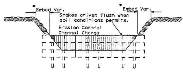
EROSION CONTROL CHANNEL CHANGE
