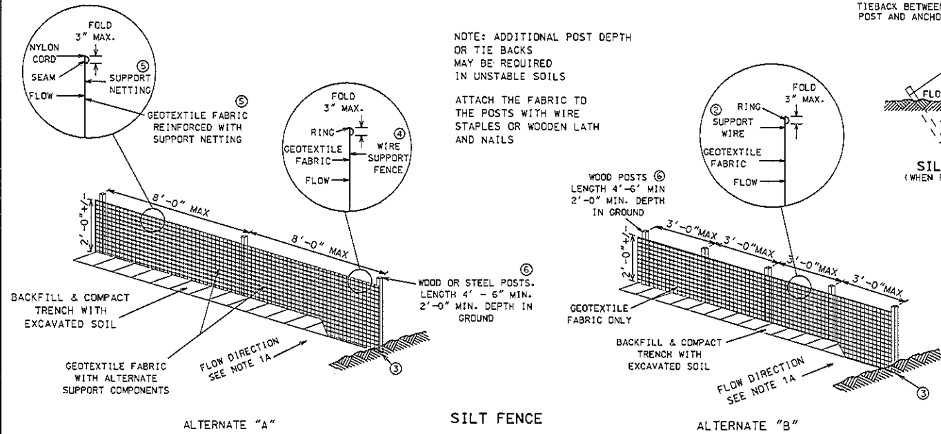
SILT FENCE AT MEDIAN SURFACE DRAINS
