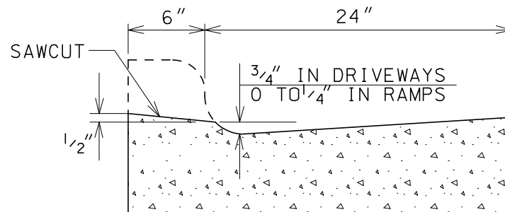
DRIVEWAY SECTION TYPE 'A' CONCRETE CURB & GUTTER
