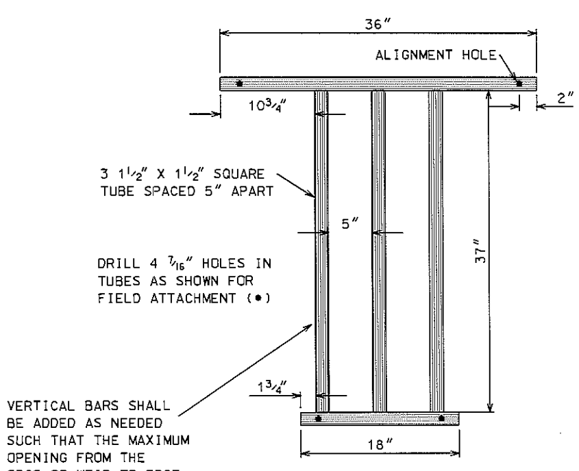
WEIR PIPE GATE
