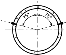
TRANSVERSE SECTION
