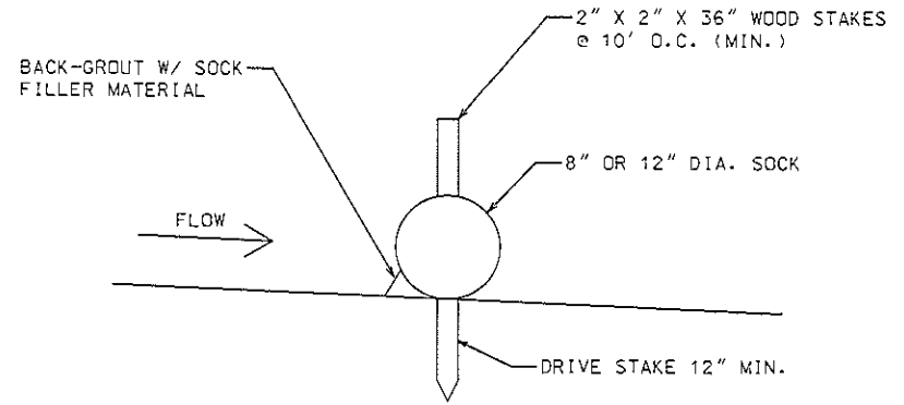
SECTION VIEW
