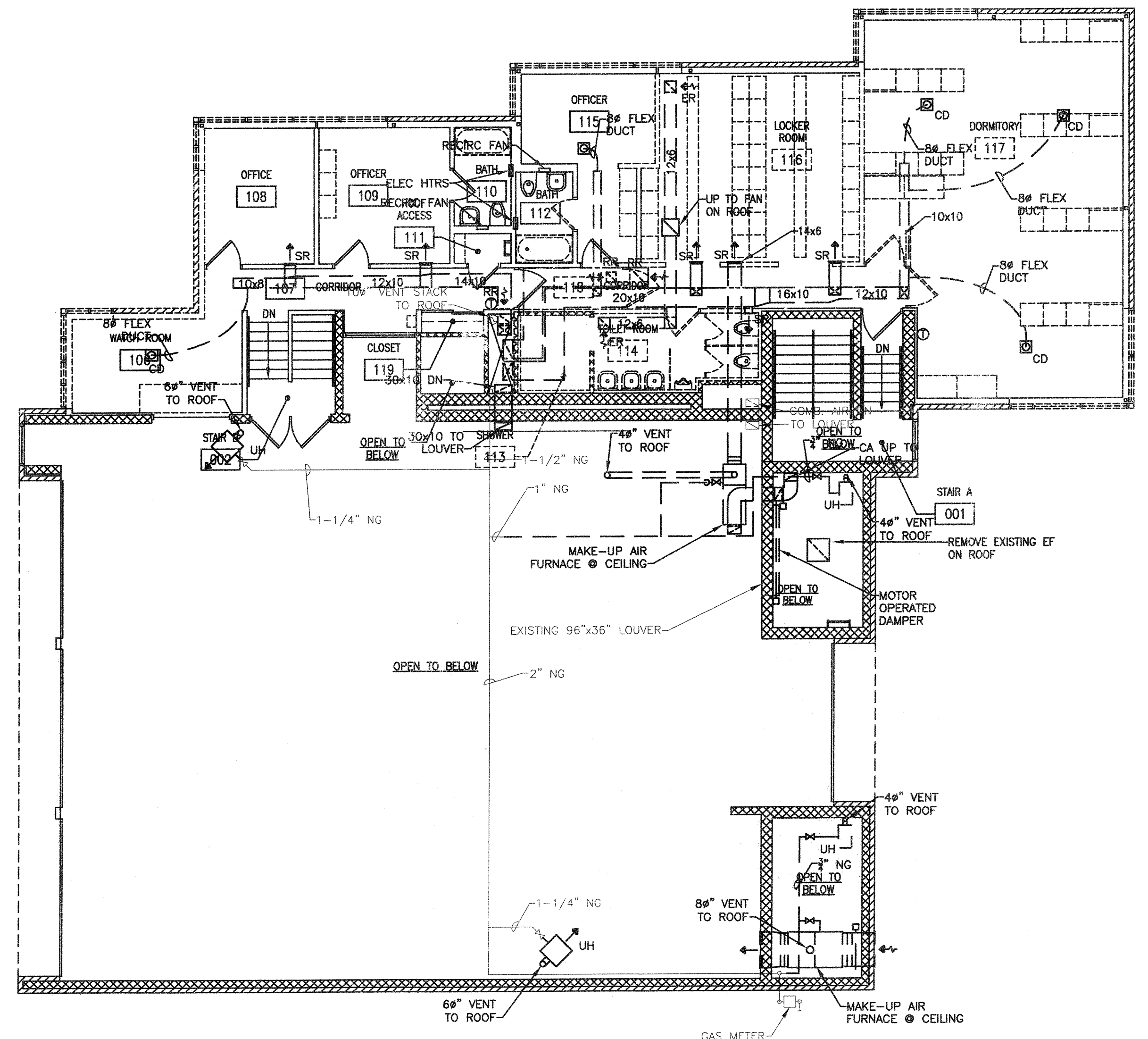
2 M101 UPPER LEVEL MECHANICAL DEMOLITION PLAN SCALE: 1/8" = 1'-0"
