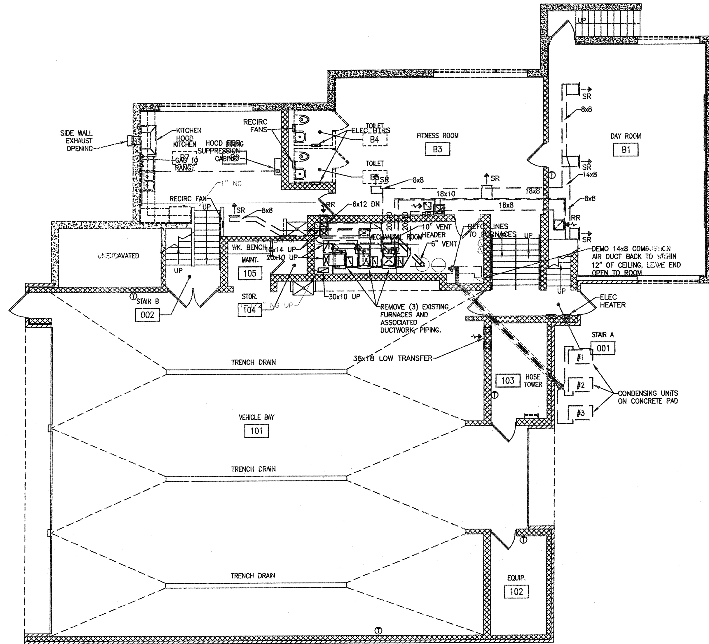
1 M101 LOWER LEVEL MECHANICAL DEMOLITION PLAN SCALE: 1/8" = 1'-0"
