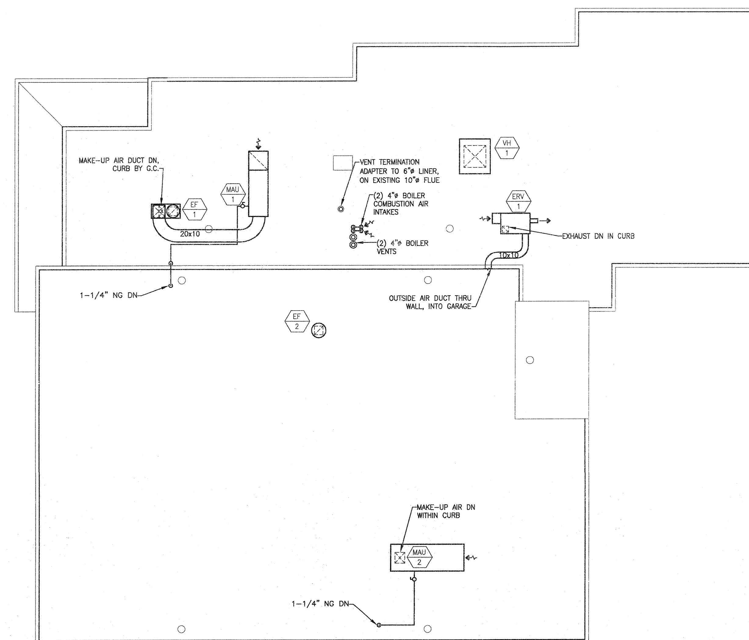
3 M202 ROOF HVAC REMODELING PLAN SCALE: 1/8" = 1'-0"
