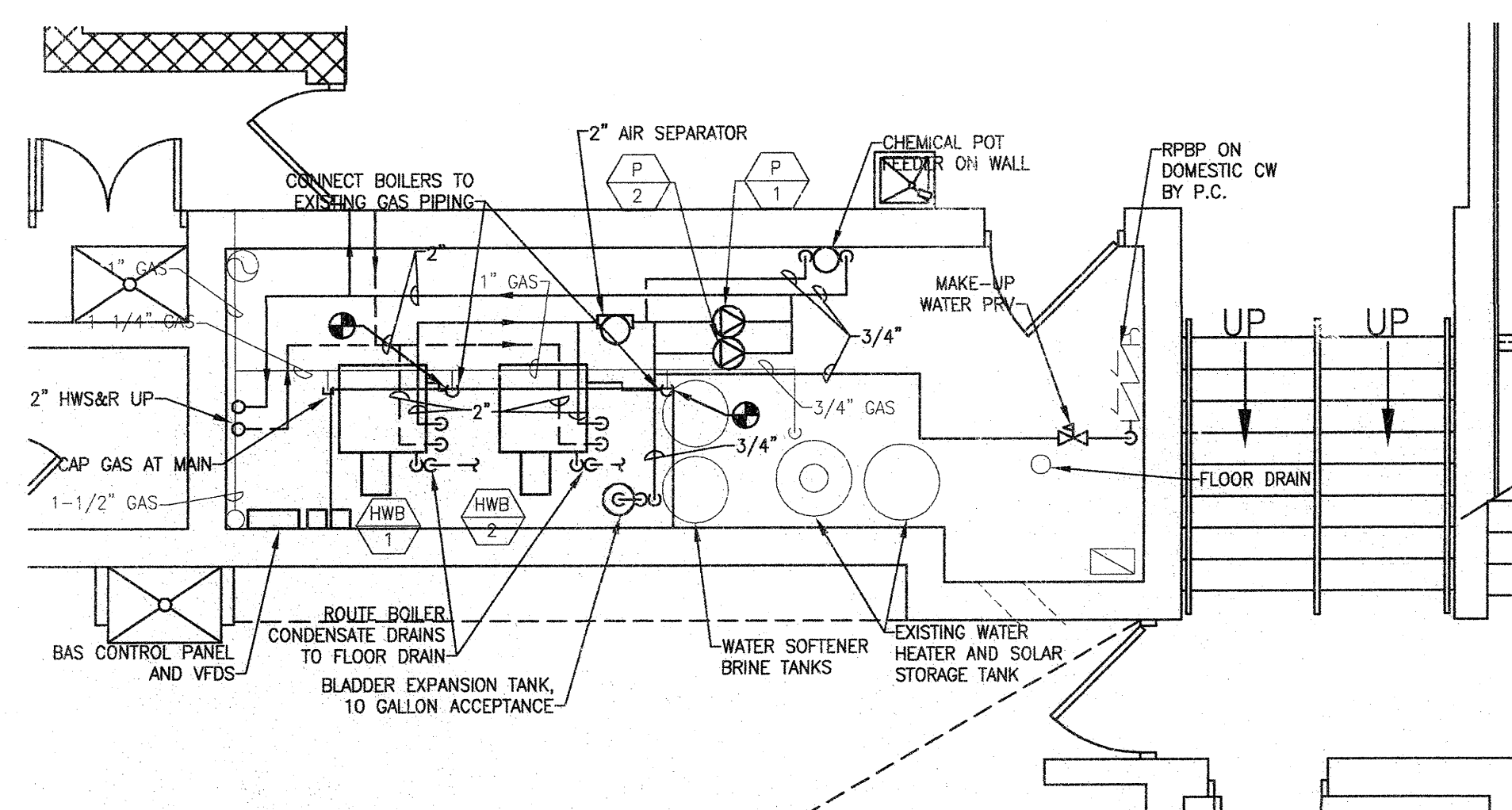
1 M202 MECH ROOM EXPANDED PIPING PLAN SCALE: 1/4" = 1'-0"
