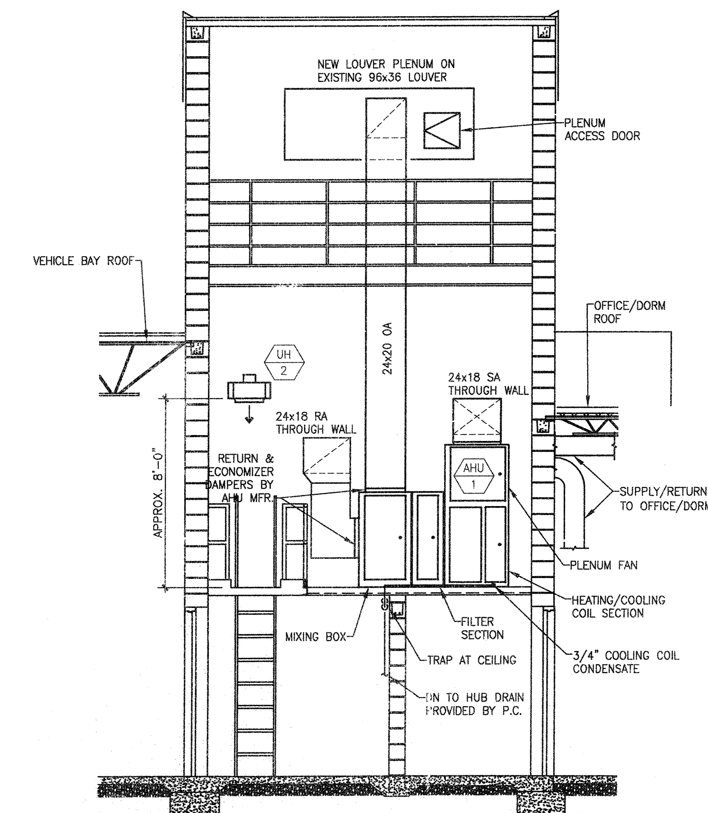
2 M202 HOSE TOWER AHU SECTION - LOOKING WEST SCALE: 1/4" = 1'-0"
