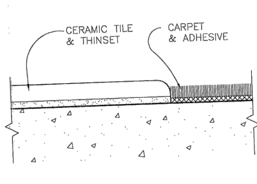
3 - Ceramic Tile to Carpet (no scale)
