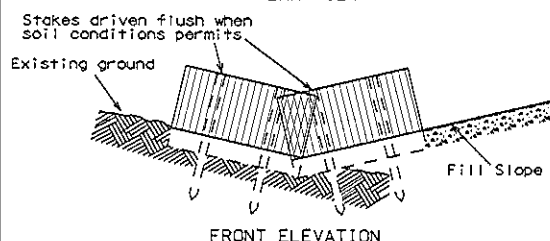
EROSION BALES AT TOE OF SLOPE WHEN EXISTING GROUND SLOPES TOWARD FILL SLOPE
