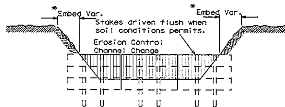
EROSION CONTROL CHANNEL CHANGE
