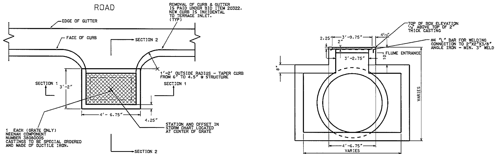
STRUCTURE
