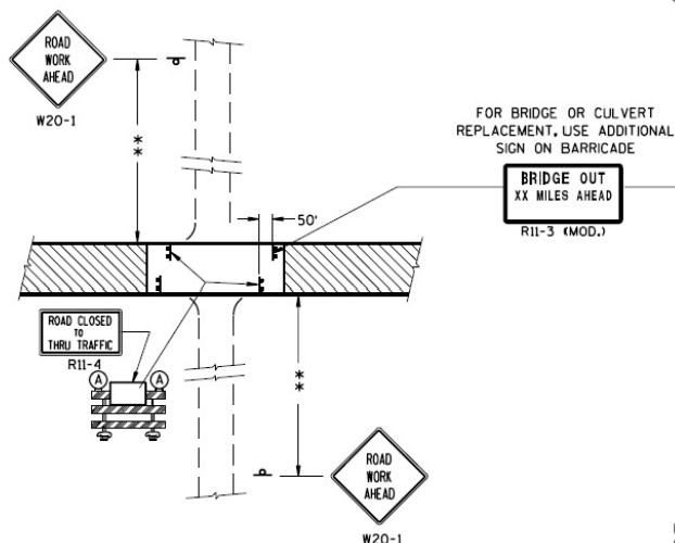
DETAIL 3 (PUBLIC CROSS-TRAFFIC MAINTAINED. CONTRACTOR, LOCAL BUSINESS AND RESIDENT ACCESS).
