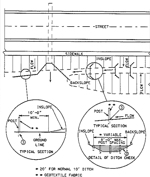
PLAN VIEW
