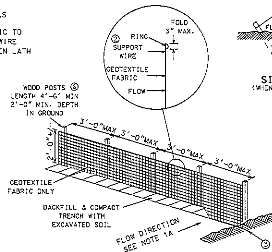
ALTERNATE "B"
