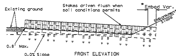
EROSION BALES AT TOE OF SLOPE
