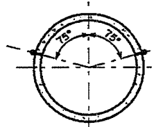
TRANSVERSE SECTION
