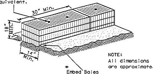
DETAIL OF EROSION BALE INSTALLATION
