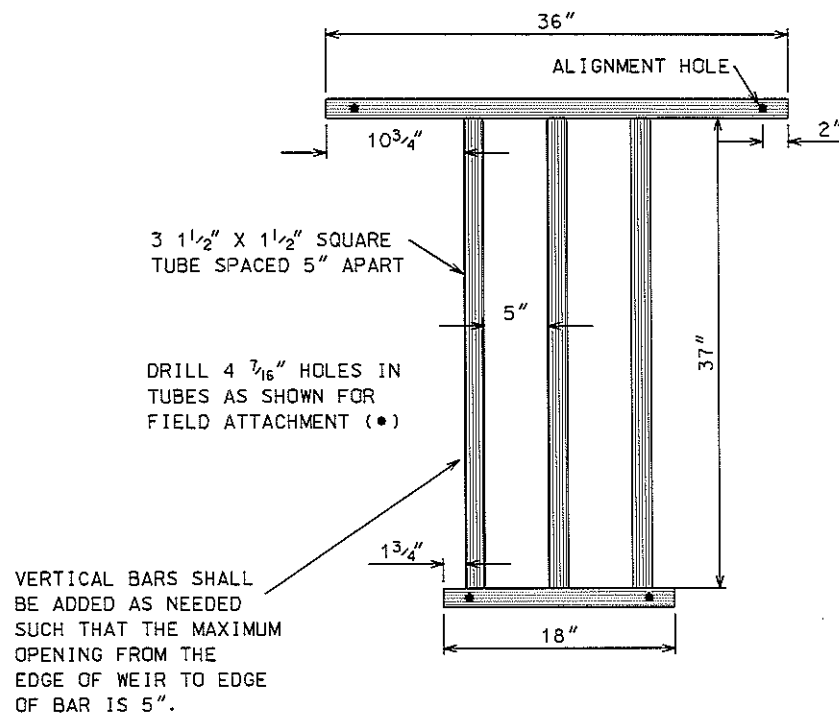
WEIR PIPE GATE
