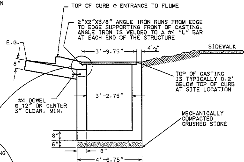
SECTION 2
