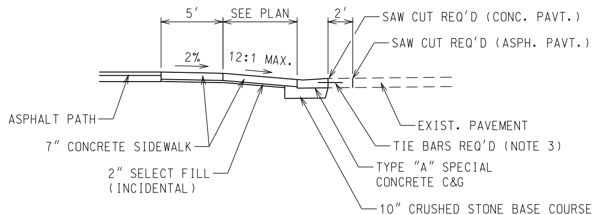
BIKE PATH RAMP SECTION A-A
