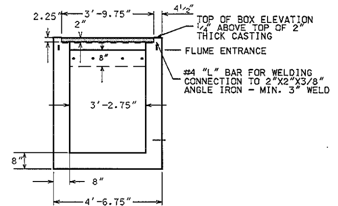
SECTION 1
