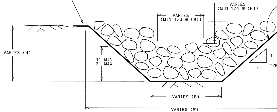
SECTION VIEW
