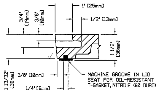
T-SEAL GASKET / CONCEALED PICK DETAIL
