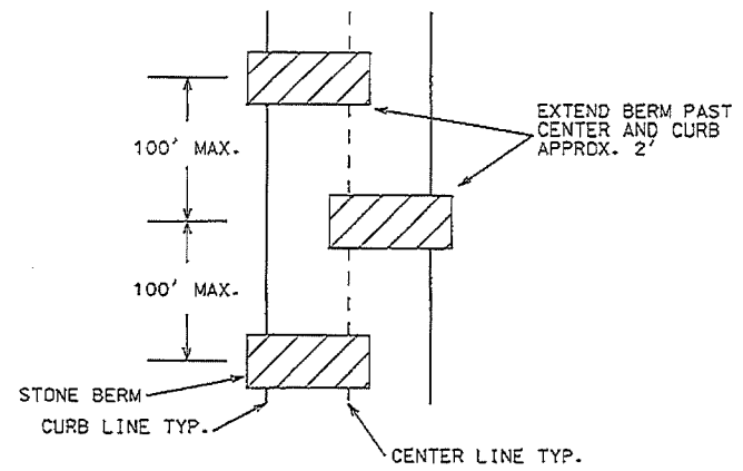
STAGGERED SPACING
