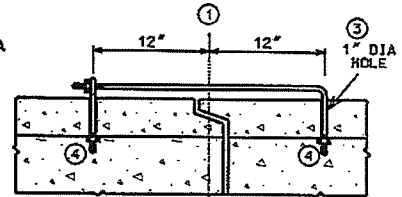
(TONGUE AND GROOVE PIPE) LONGITUDINAL SECTION
