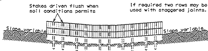
FRONT ELEVATION
