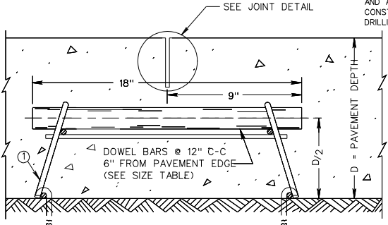
DOWELED CONTRACTION JOINT
