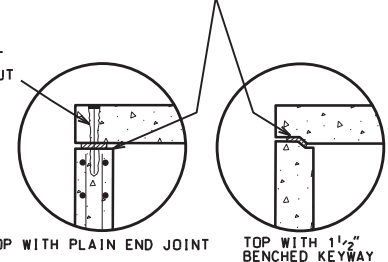
PRECAST TOP SLAB JOINT DETAIL
