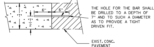
SECTION A-A PAVEMENT TIES
