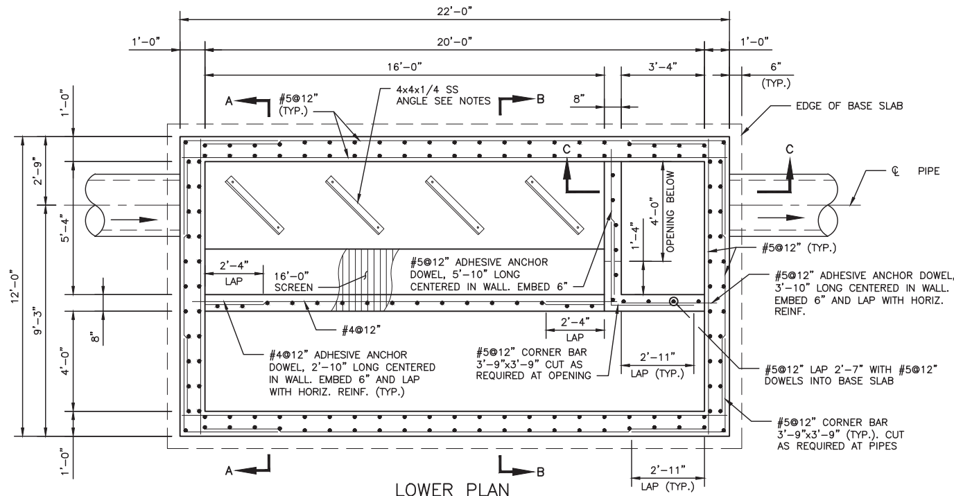
LOWER PLAN
