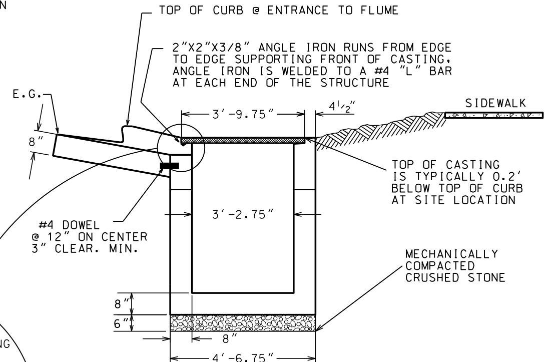
SECTION 2
