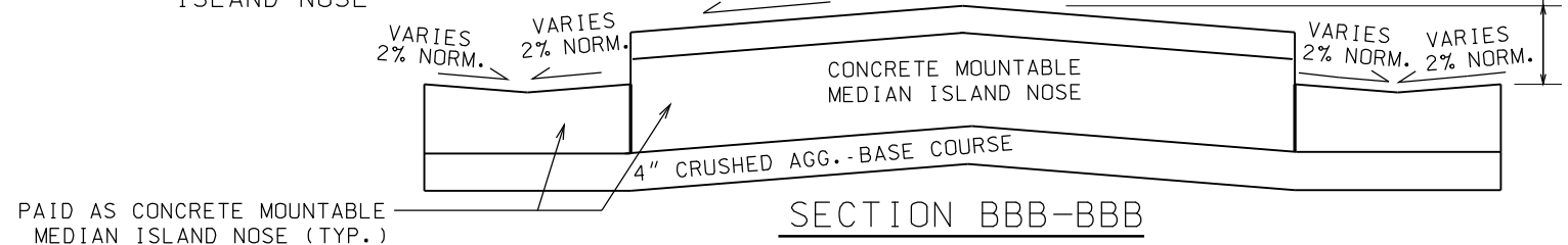
DETAIL CONCRETE MOUNTABLE MEDIAN ISLAND NOSE
