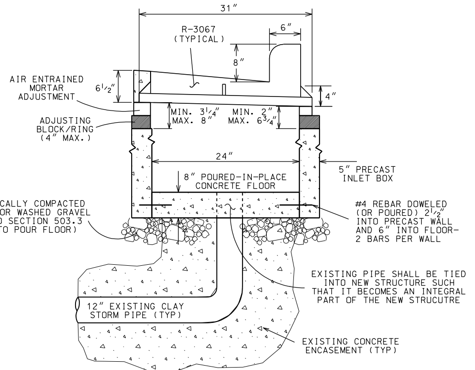
PRECAST OPTION
