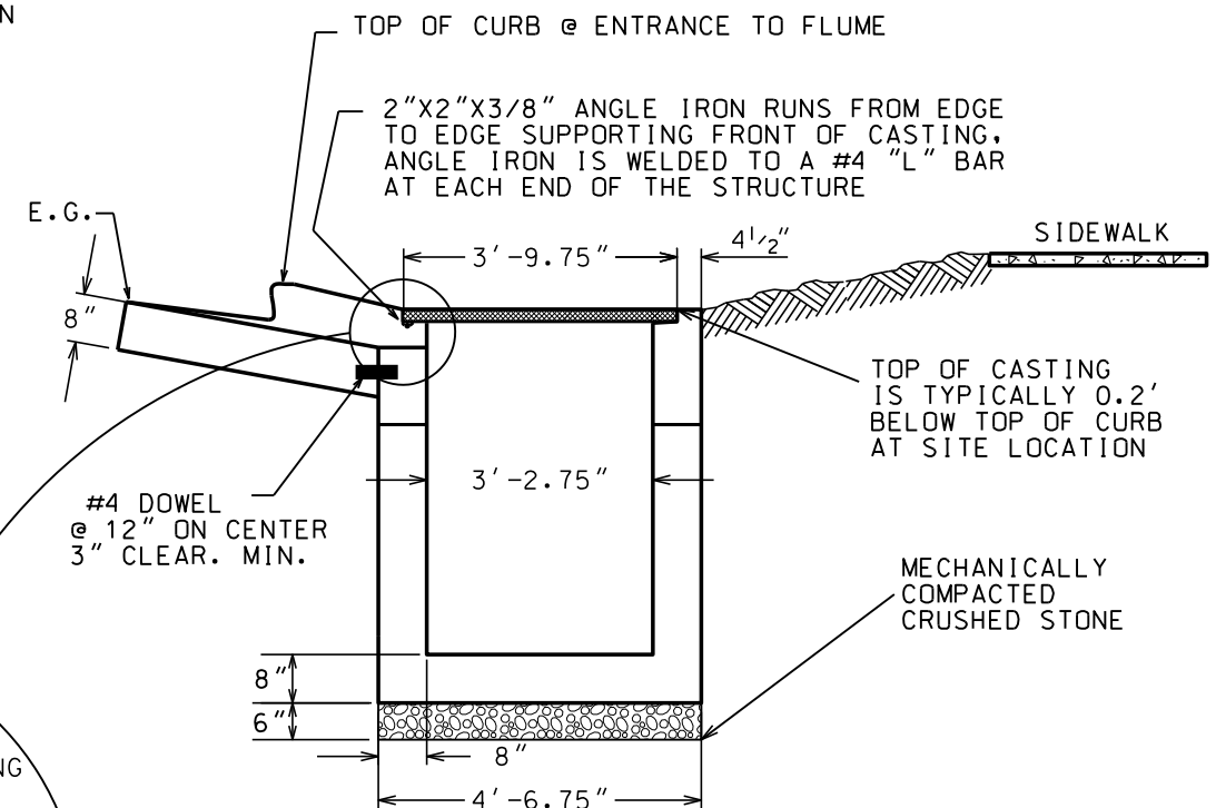
SECTION 2
