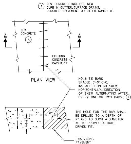
SECTION A-A PAVEMENT TIES
