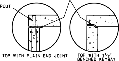
PRECAST TOP SLAB JOINT DETAIL
