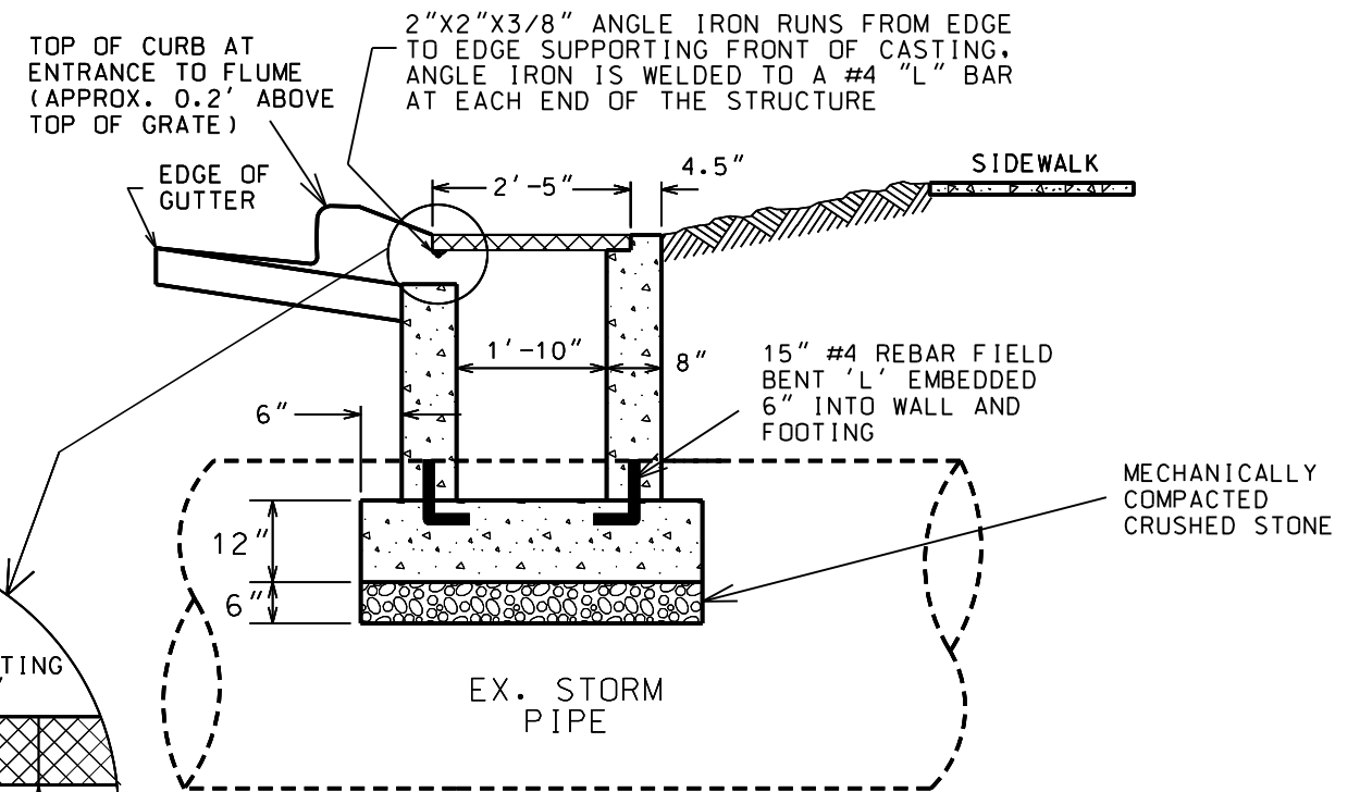
SECTION 1
