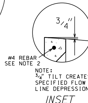
FIELD POURED FLOOR REINFORCEMENT
