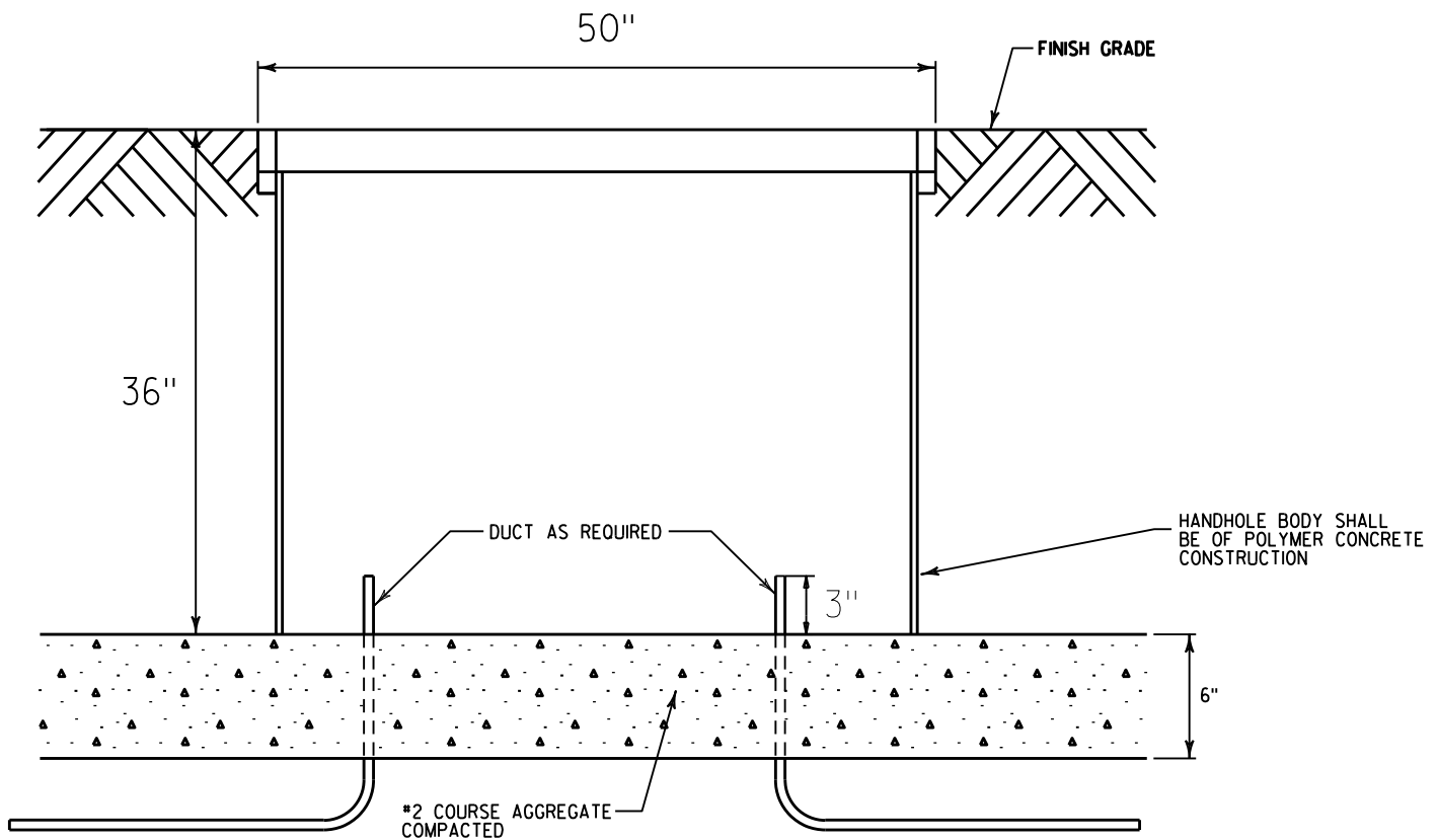
ELECTRICAL PULLBOX TYPE VII
