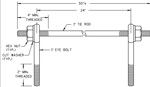
EYE BOLTS AND TIE ROD
