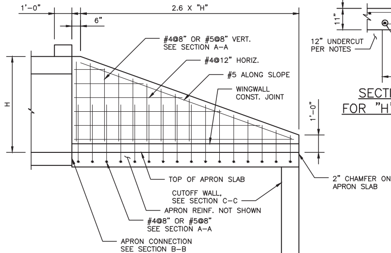
WINGWALL ELEVATION
