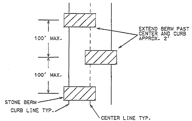
STAGGERED SPACING
