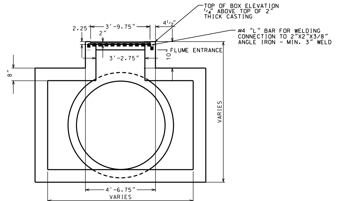
SECTION 1
