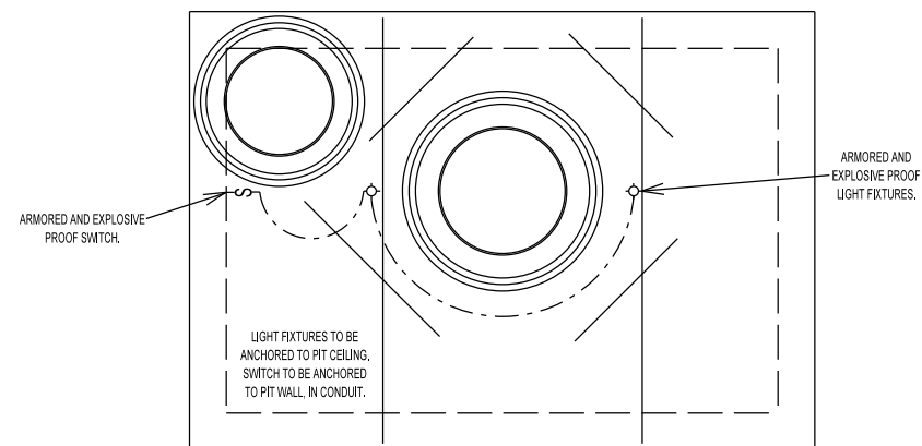
METER PIT LIGHT DETAIL
