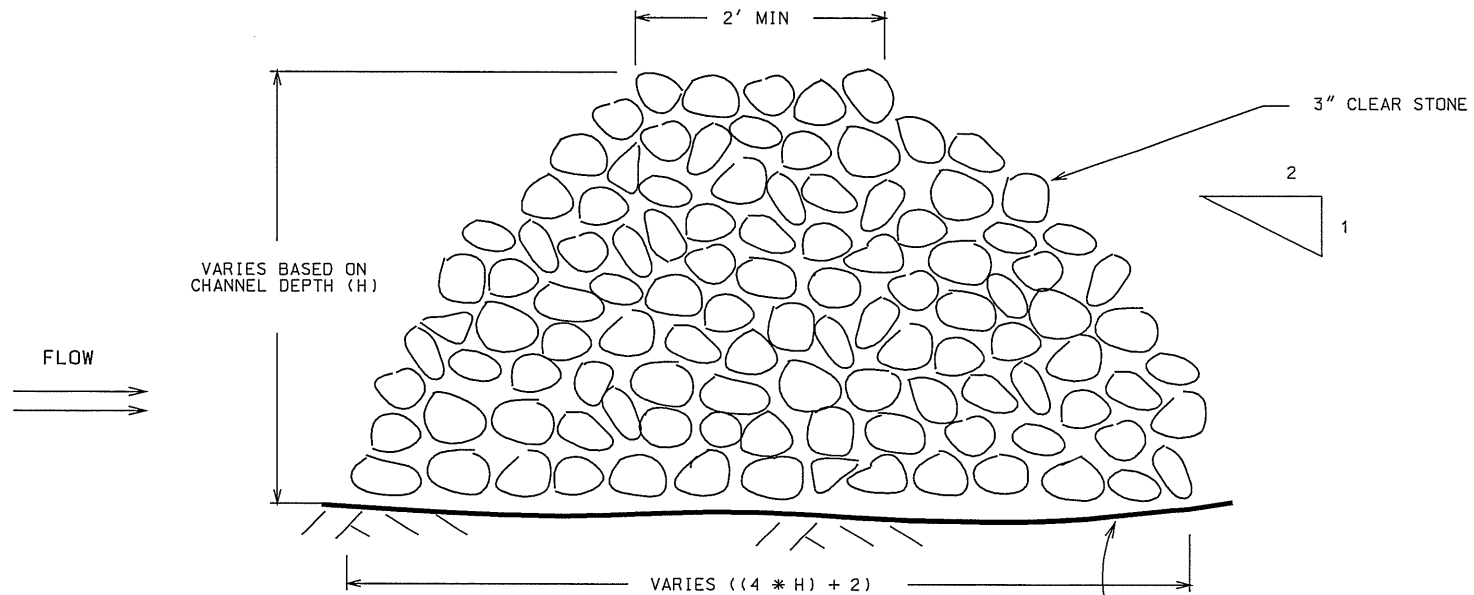
SIDE VIEW
