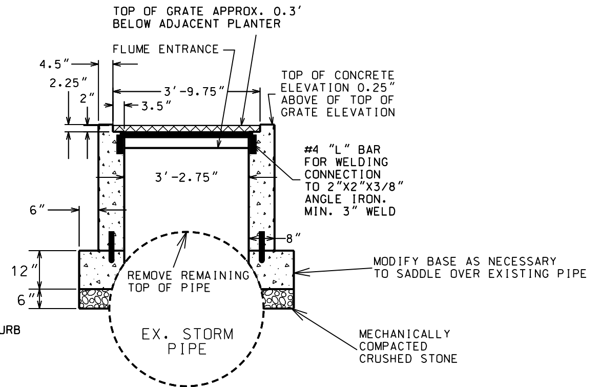
SECTION 1
