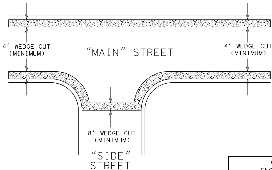
DETAIL "C" RADI' RETURN CUTS
