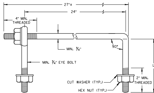
EYE BOLT AND TIE ROD
