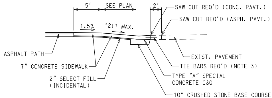
BIKE PATH RAMP SECTION A-A
