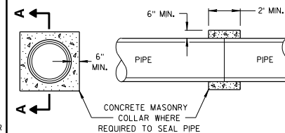
SECTION A-A CONCRETE COLLAR DETAIL
