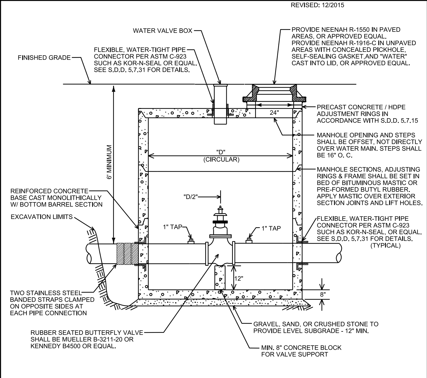
WATER VALVE MANHOLE
