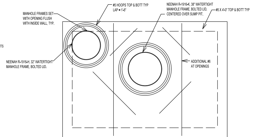
METER PIT ROOF DETAIL
