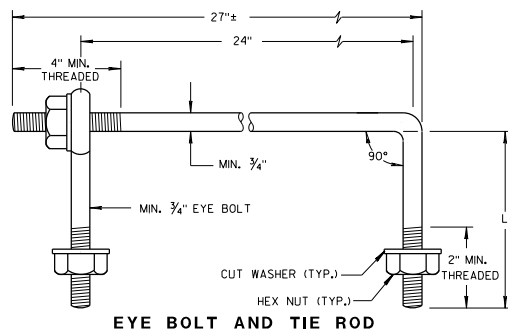
EYE BOLT AND TIE ROD
