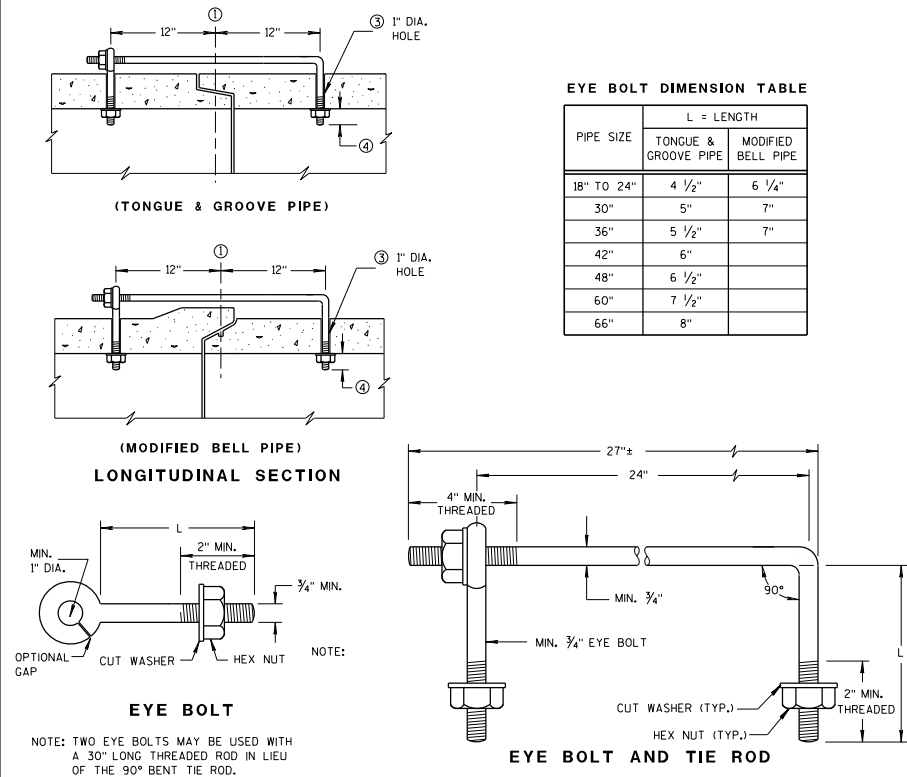
(JOINT TIES FOR 18" TO 66" DIA. CONCRETE PIPE) EYE BOLT AND TIE ROD ASSEMBLY (ALTERNATE NO. 2)
