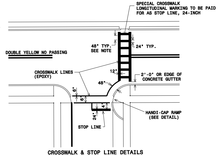
CROSSWALK & STOP LINE DETAILS
