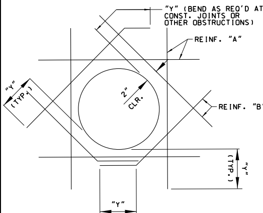
PRECAST TOP SLAB JOINT DETAIL
