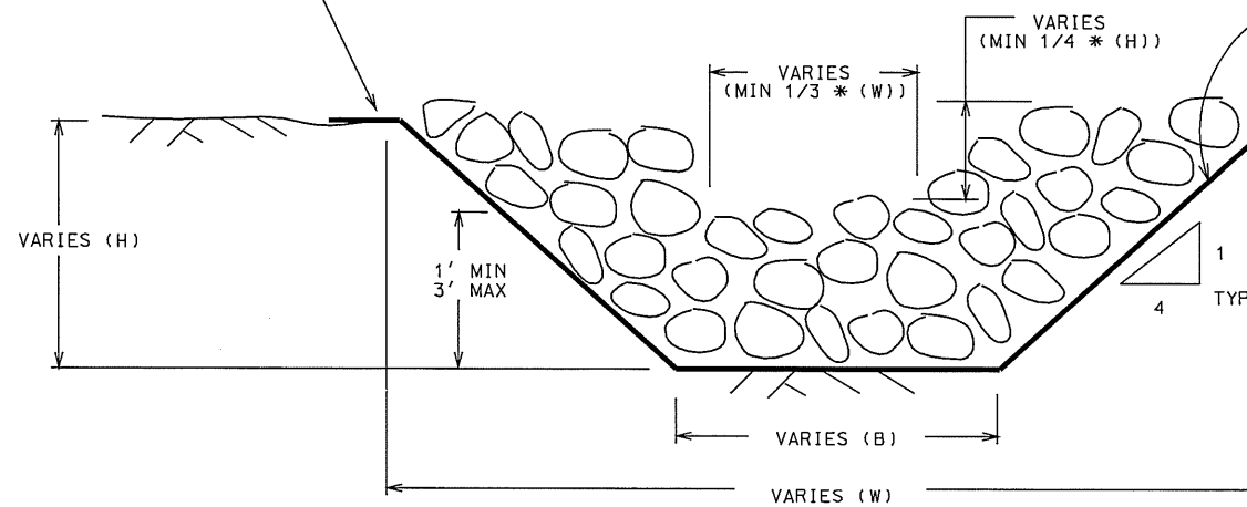
SECTION VIEW
