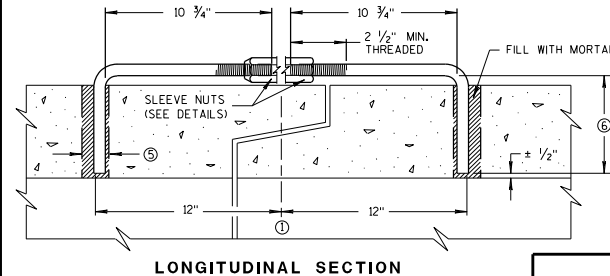
CONCRETE COLLAR DETAIL
