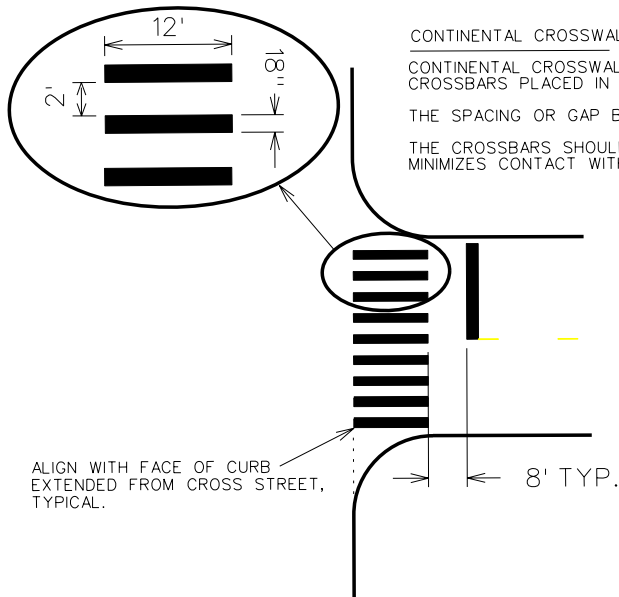
CONTINENTAL X-WALK & STOP LINES DETAIL
