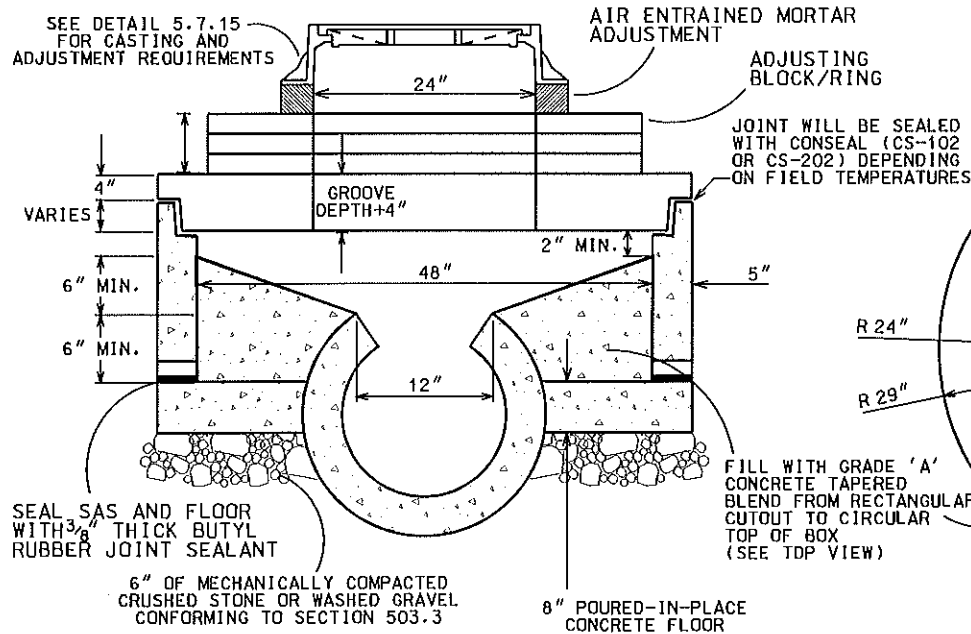
SIDE VIEW
