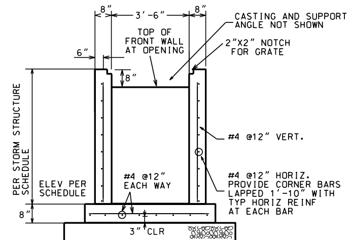
SECTION 1
