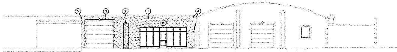
NEW SOUTH ELEVATION 12.11.17
