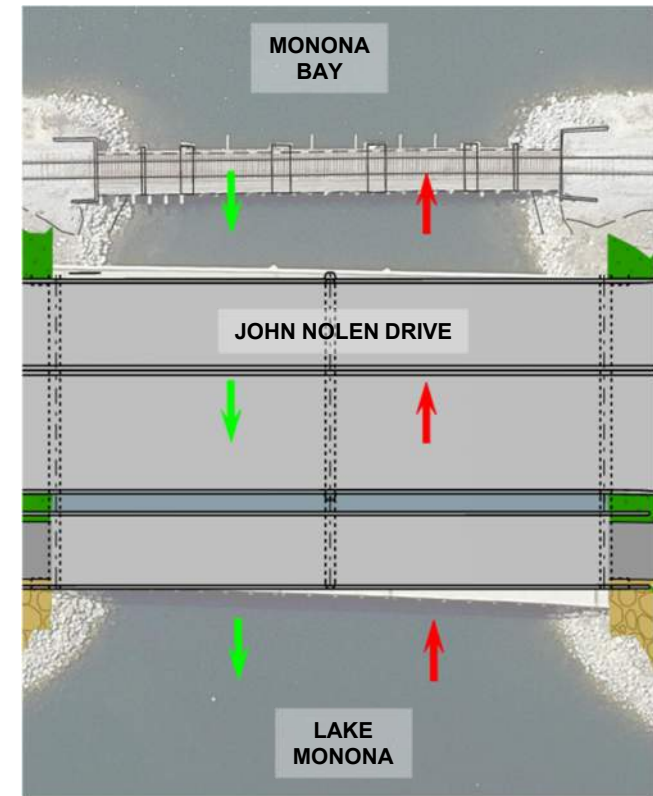
AFTER CONSTRUCTION (SEPARATE OWN SPAN)
