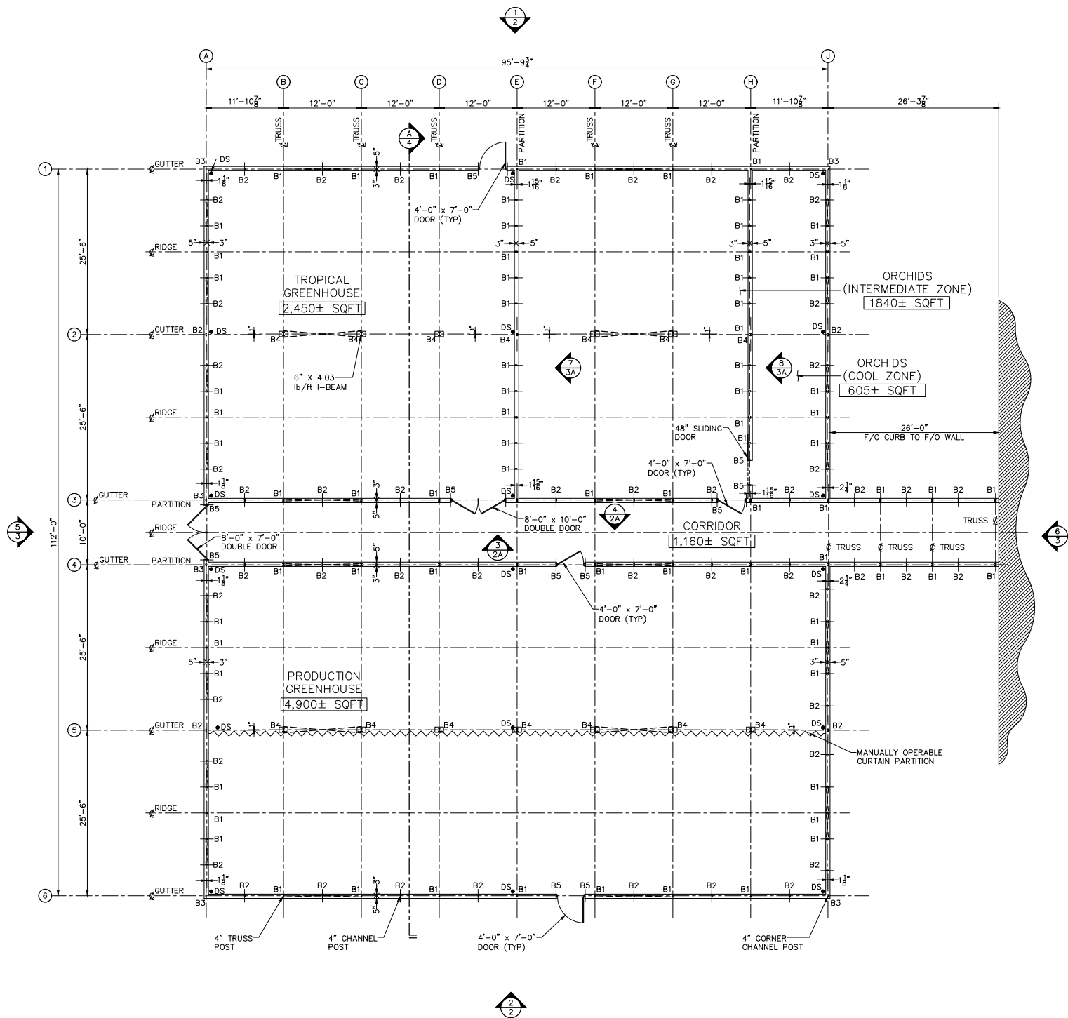
greenhouse floor plan
