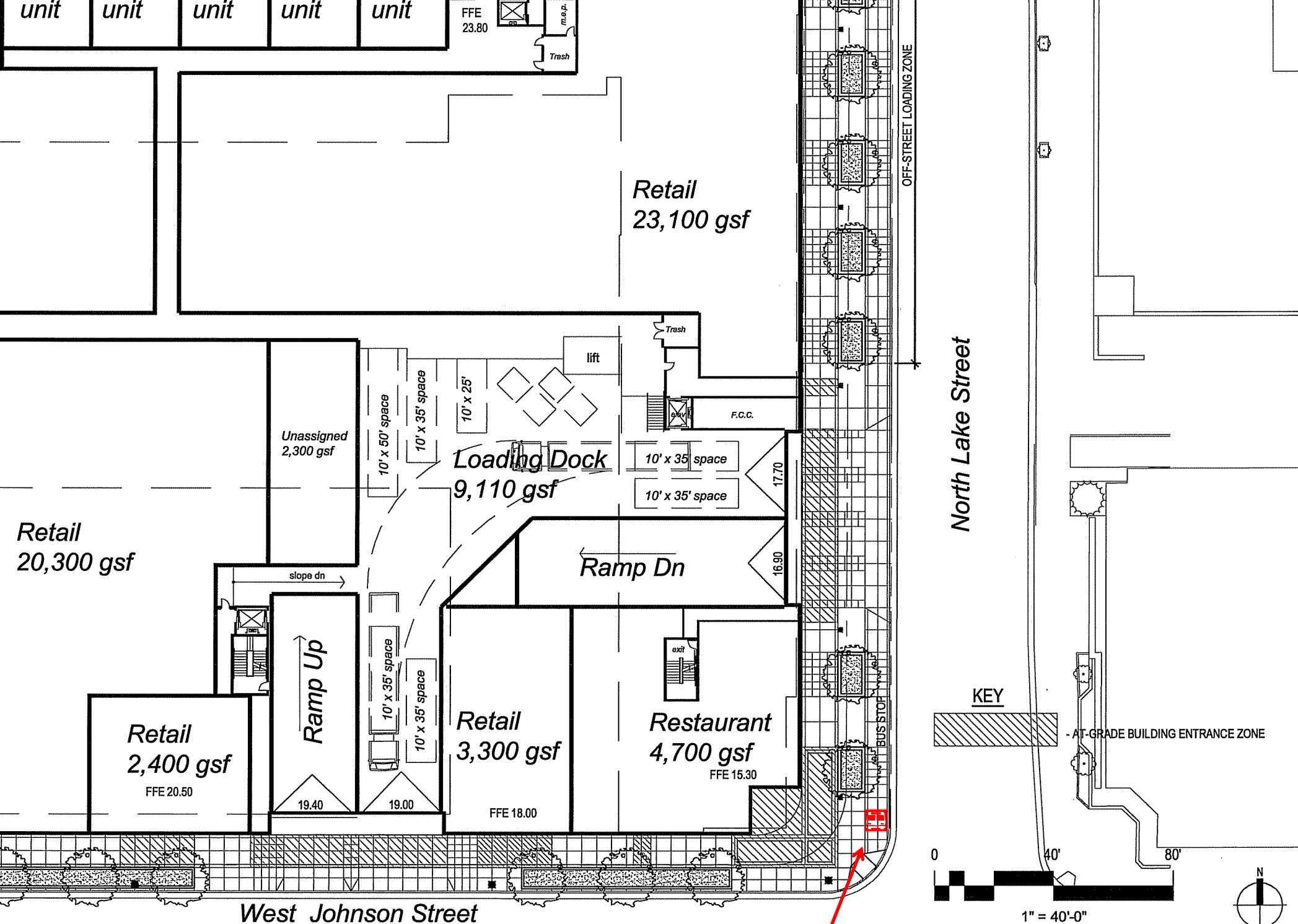
First Floor and Site Plan
