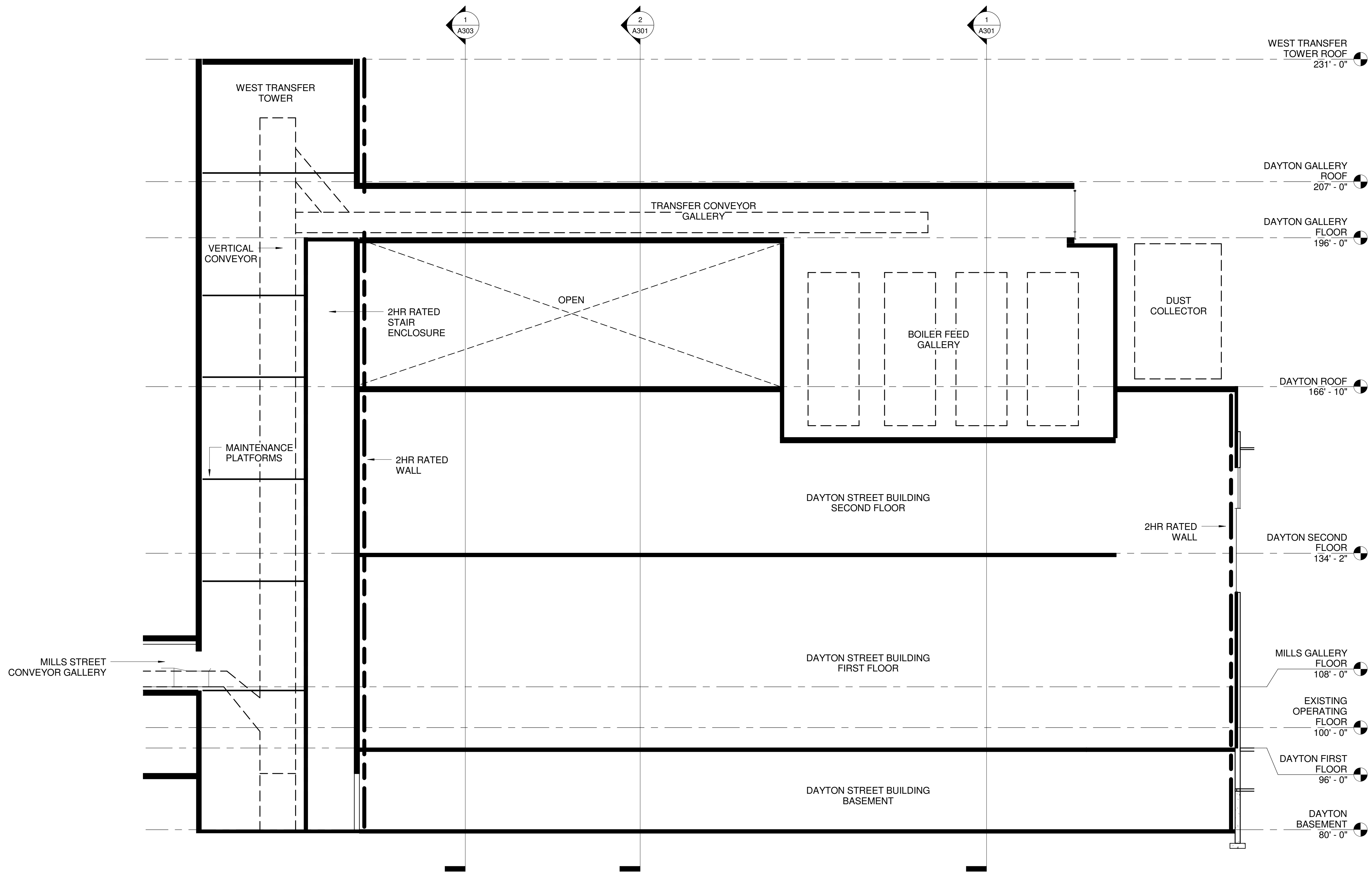
3 DAYTON STREET BUILDING SECTION A302 3/32" = 1'-0"
