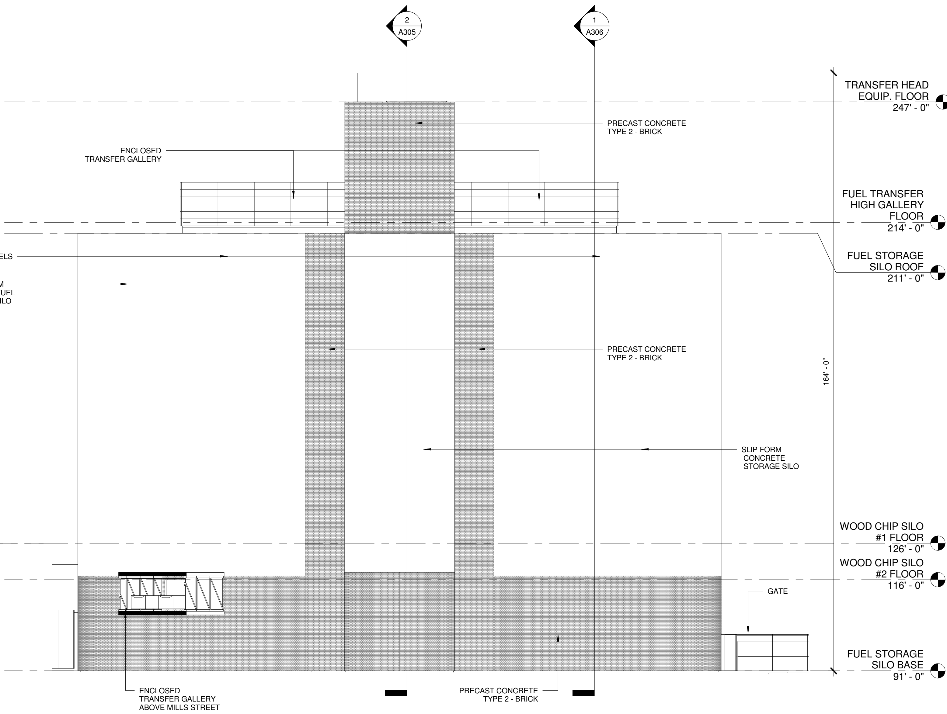
1 FUEL STORAGE - WEST ELEVATION (MILLS STREET) A204 1/16" = 1'-0"
