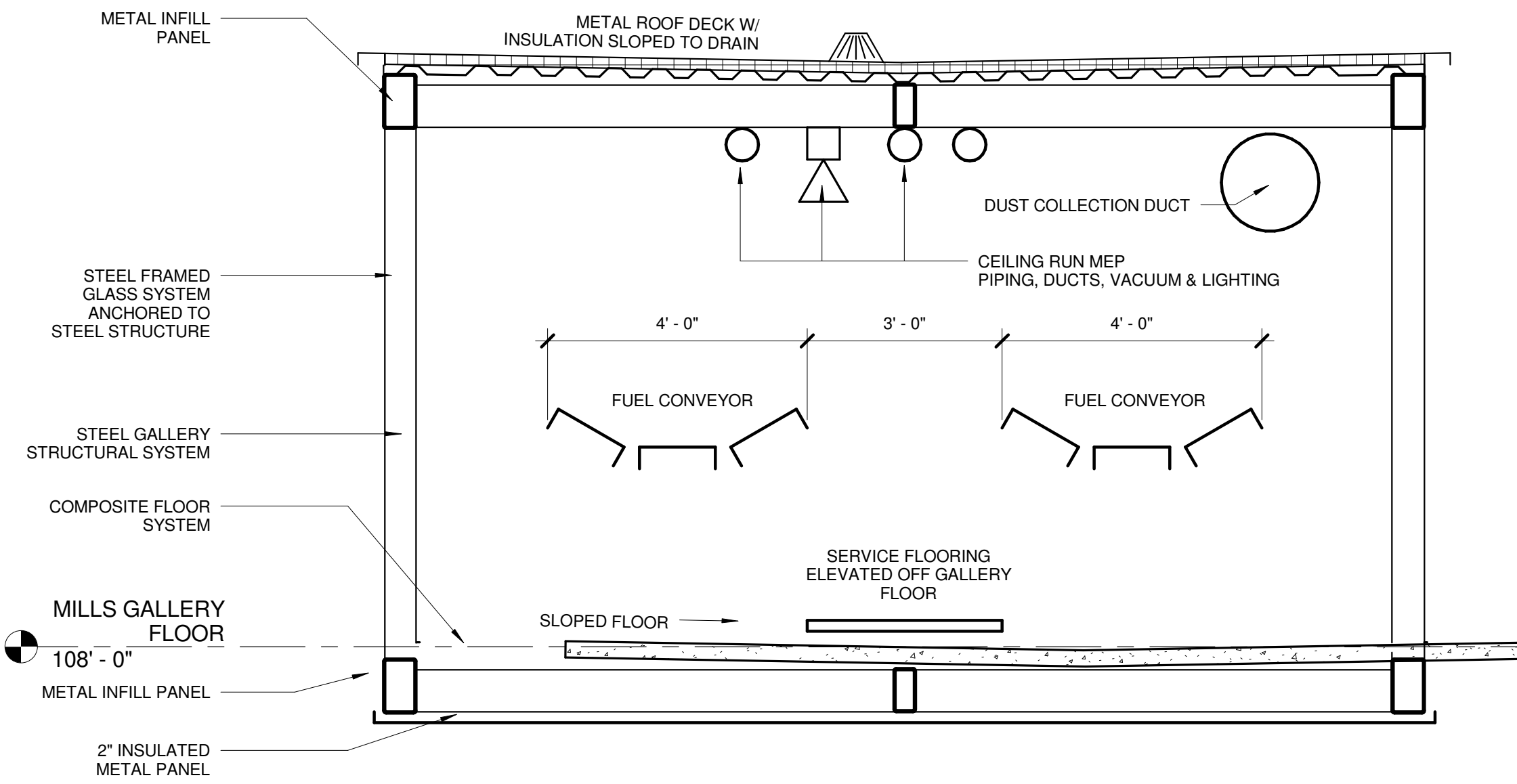
2 MILLS STREET GALLERY SECTION A311 1/2" = 1'-0"
