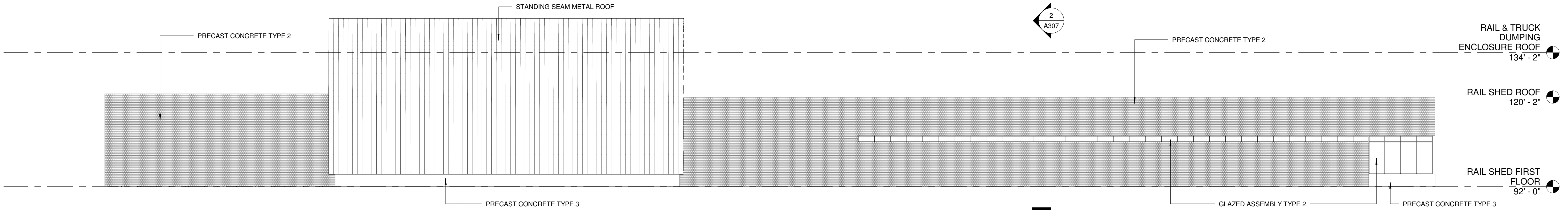
1 RAIL SHED & HOPPER - NORTH ELEVATION A206 1/16" = 1'-0"
