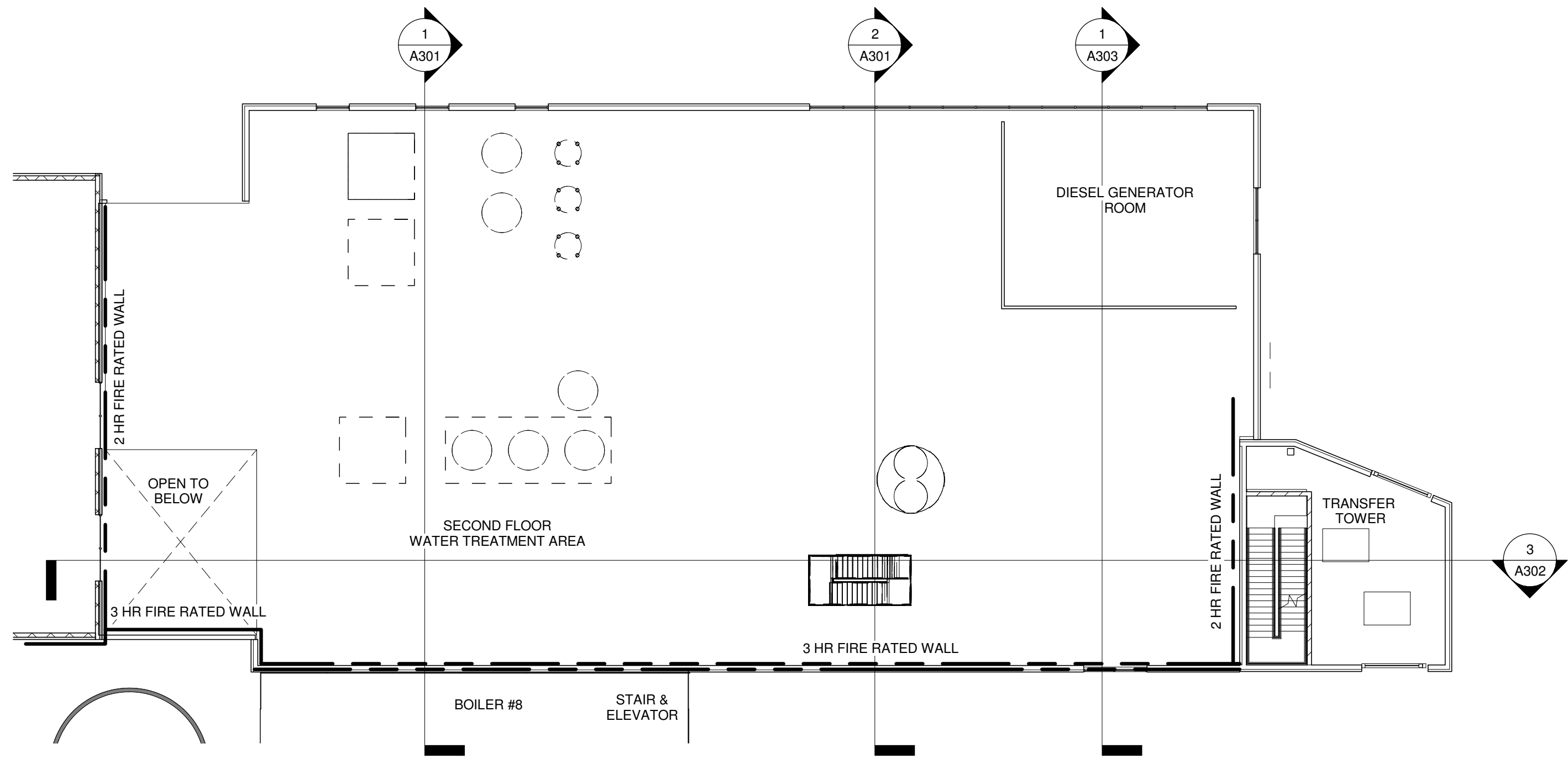
3 DAYTON STREET BUILDING SECOND FLOOR PLAN A101 1/16" = 1'-0" NORTH
