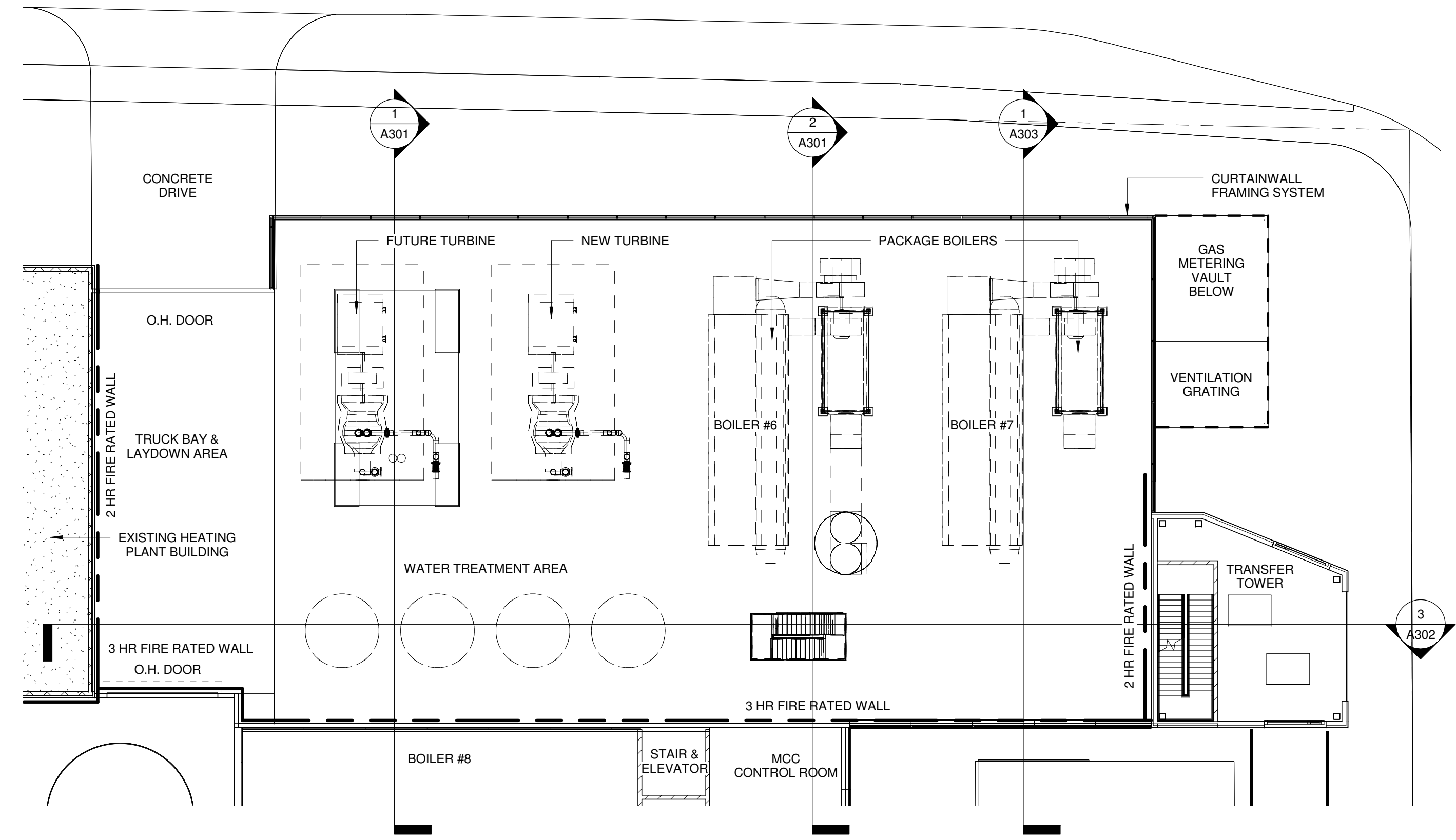
2 DAYTON STREET BUILDING - FIRST FLOOR PLAN A101 1/16" = 1'-0" NORTH
