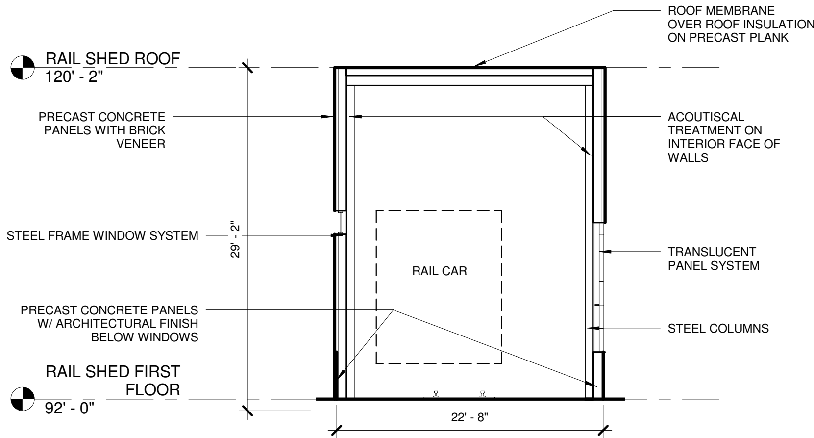
2 RAIL SHED SECTION A307 1/8" = 1'-0"
