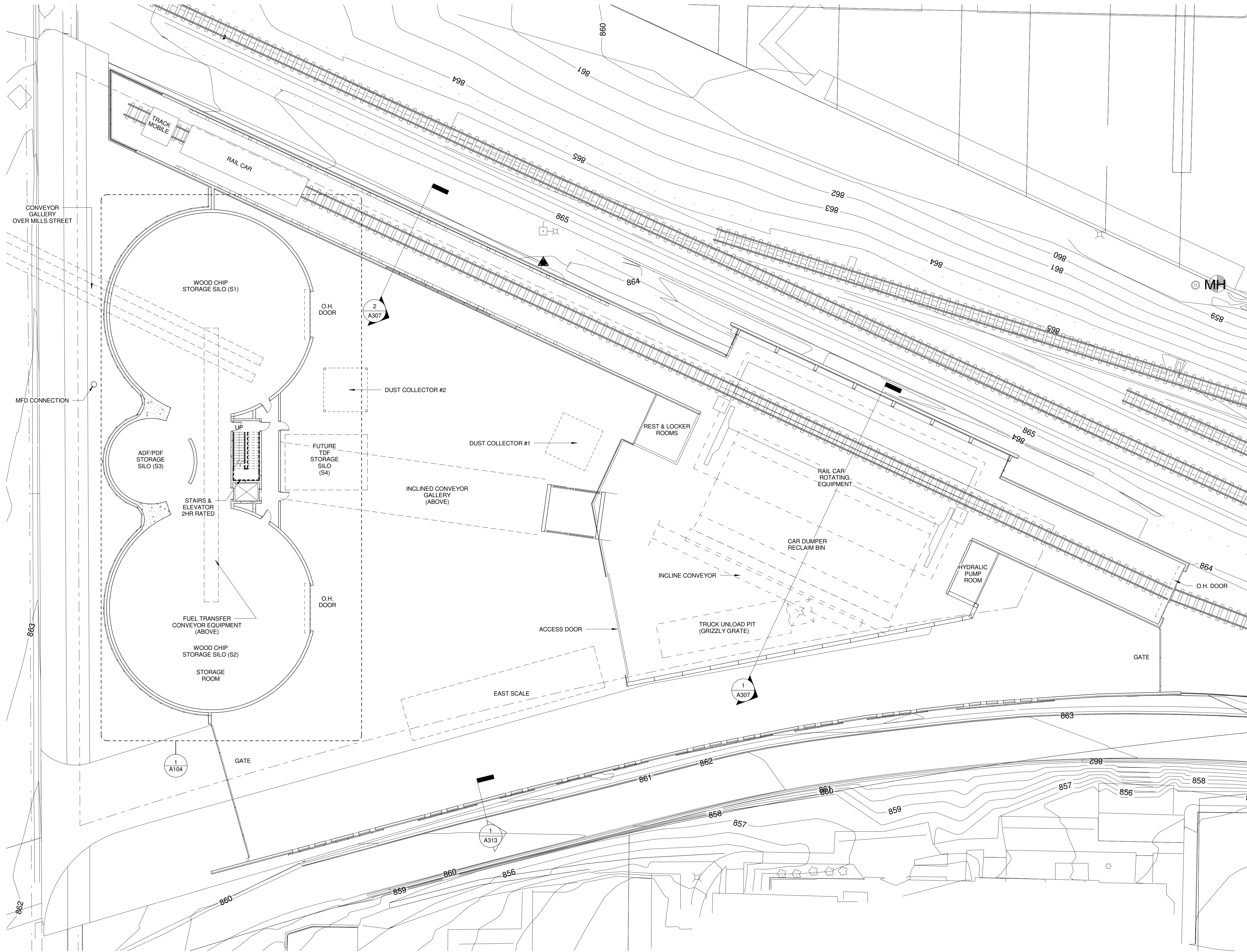
1 RAIL SHED, HOPPER & FUEL STORAGE - FIRST FLOOR PLAN A103 1/16" = 1'-0"
