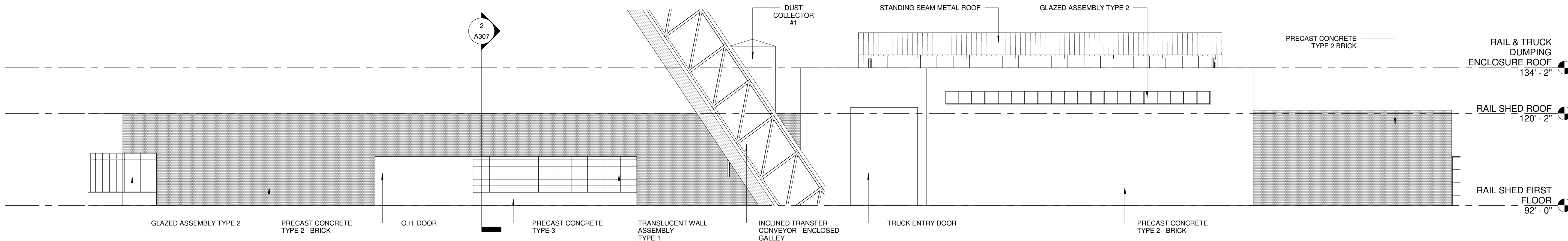
2 RAIL SHED & HOPPER SOUTH ELEVATION A206 1/16" = 1'-0"
