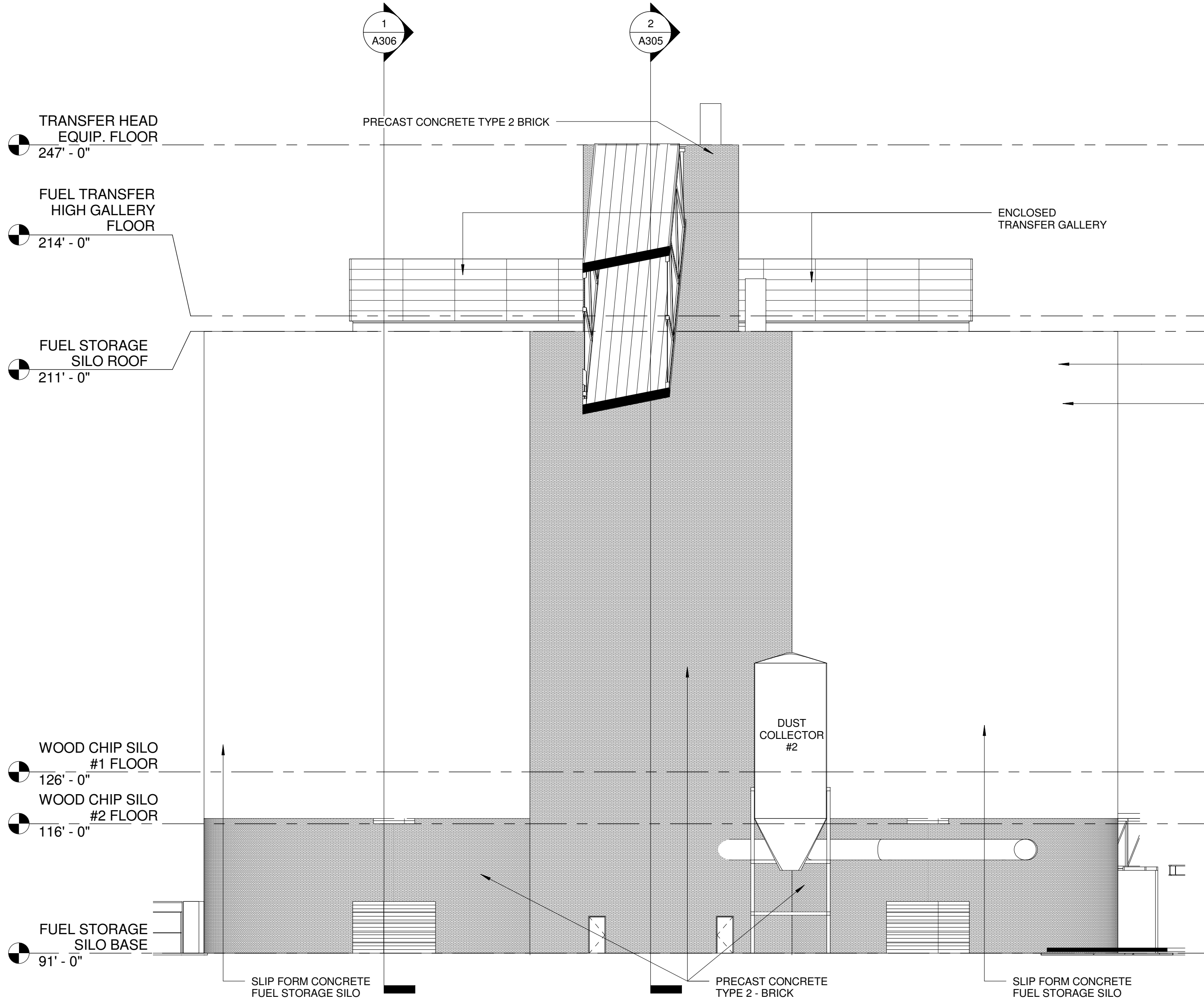
2 FUEL STORAGE - EAST ELEVATION A204 1/16" = 1'-0"
