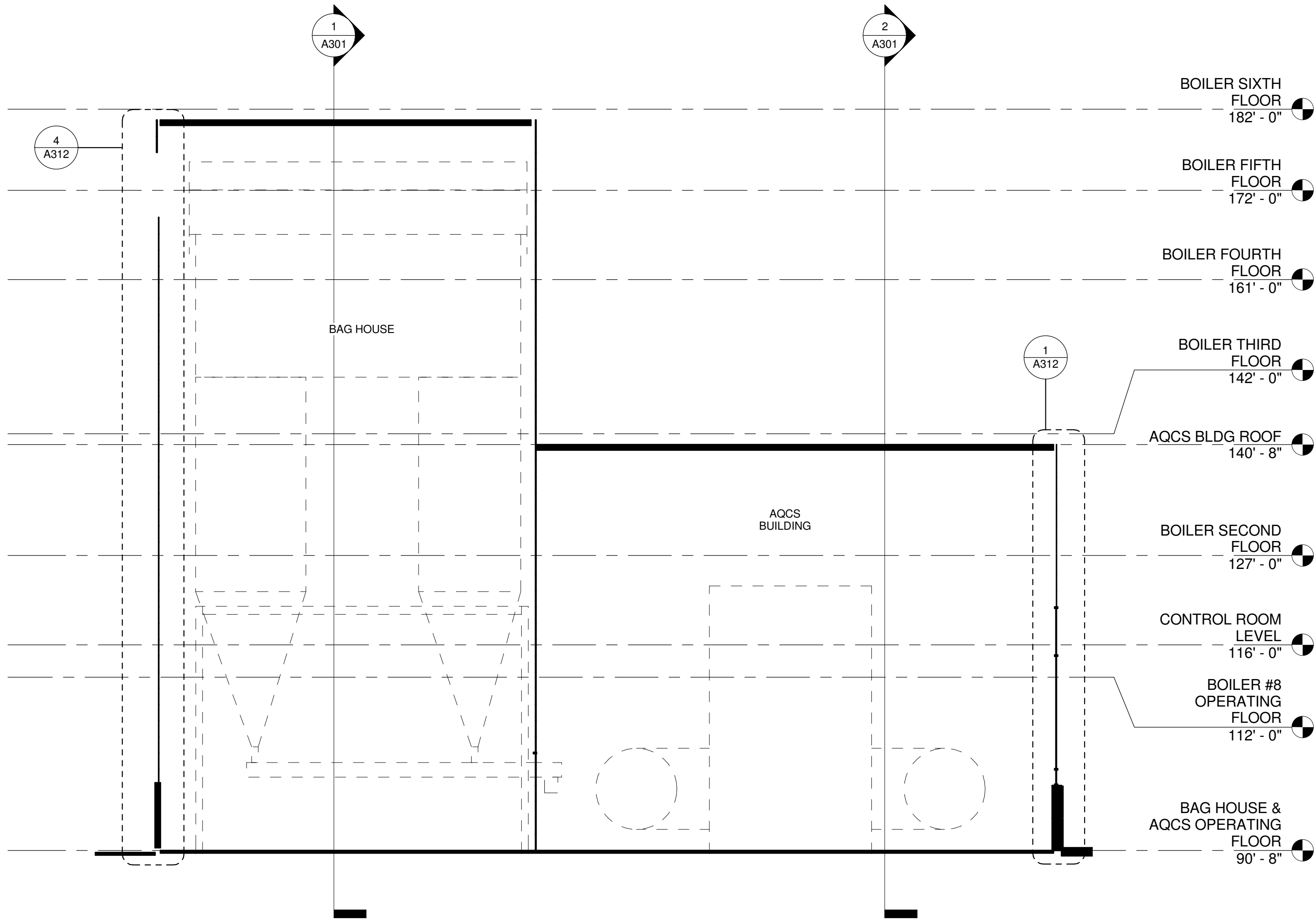
2 A304 BAG HOUSE, AIR POLLUTION CONTROL BUILDING SECTION 3/32" = 1'-0"
