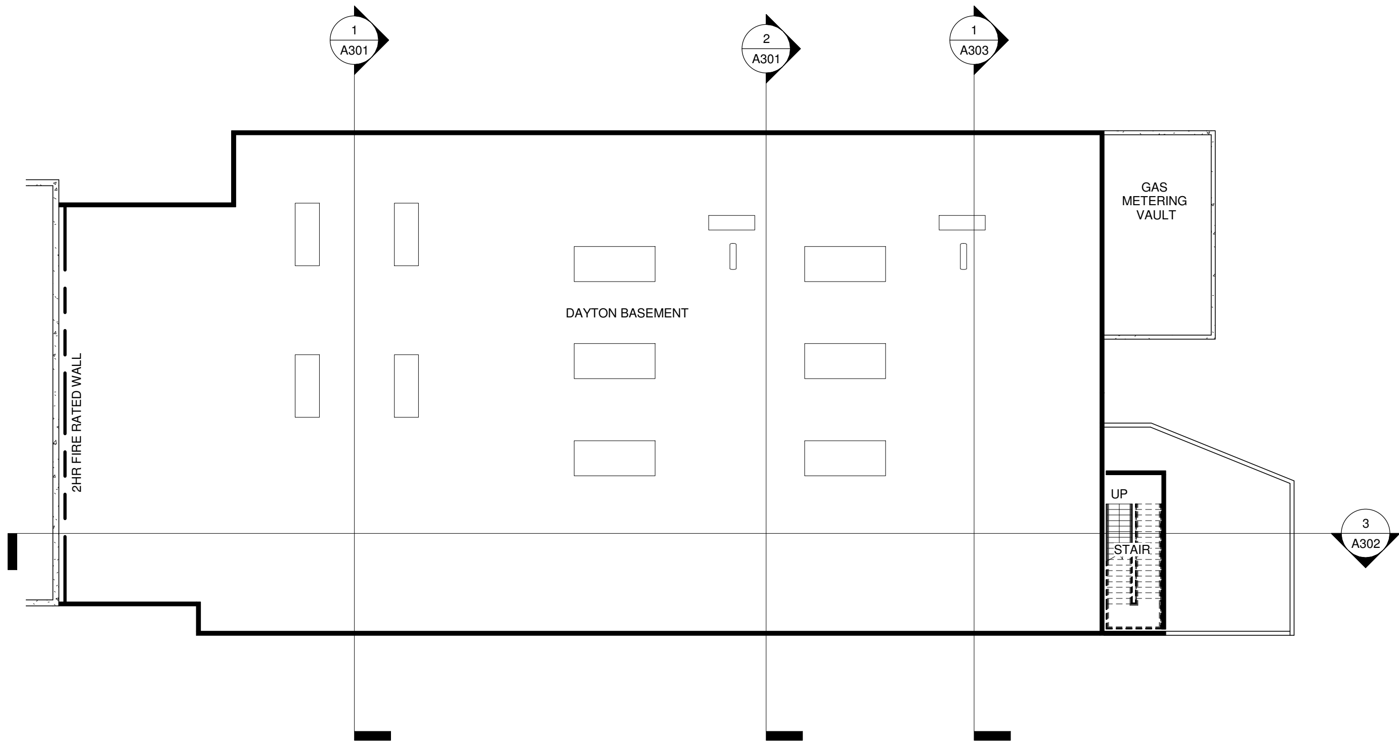
1 DAYTON STREET BUILDING BASEMENT PLAN A101 1/16" = 1'-0" NORTH
