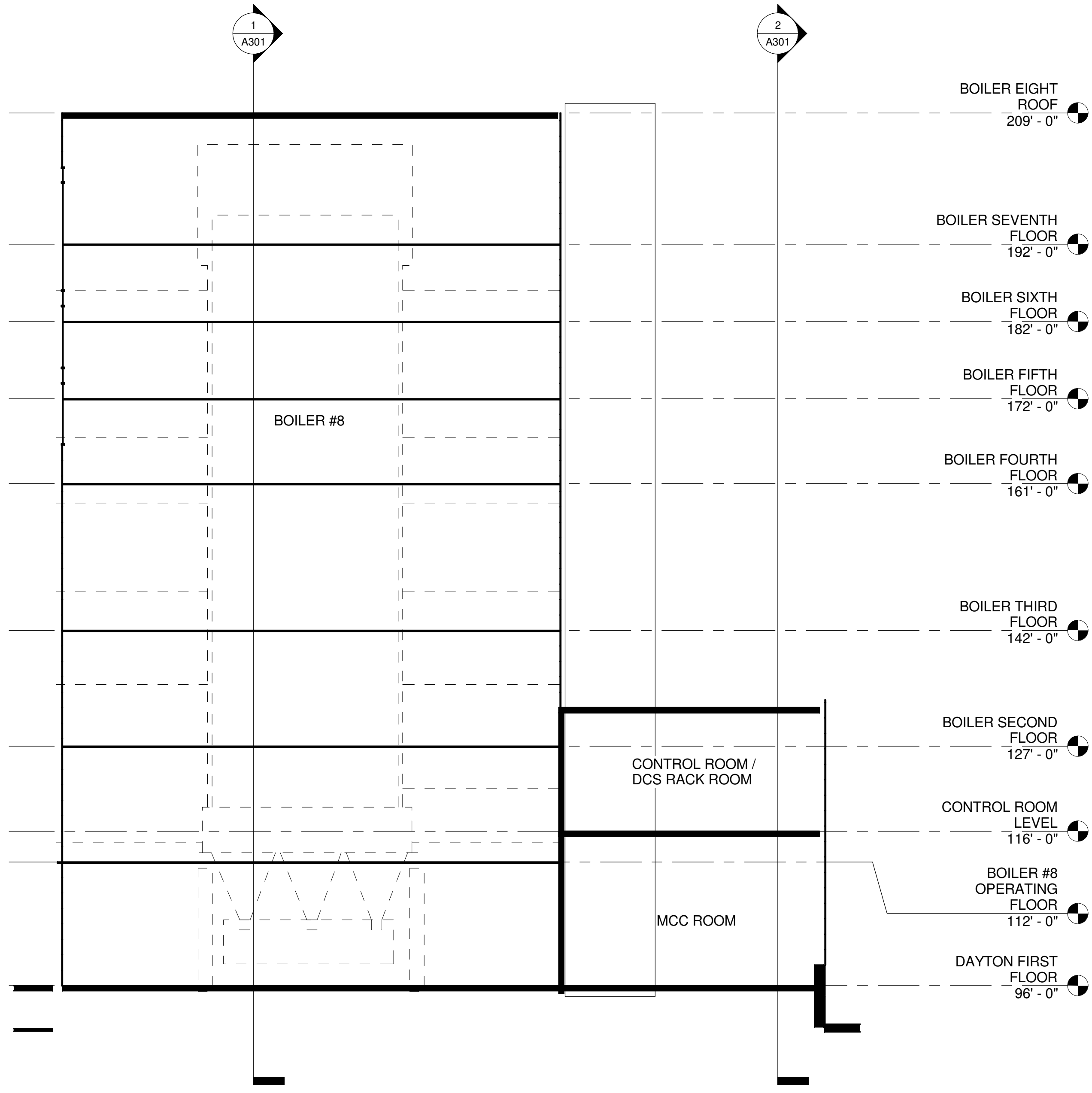
1 A304 BOILER NO. SIX / CONTROL ROOM SECTION 3/32" = 1'-0"
