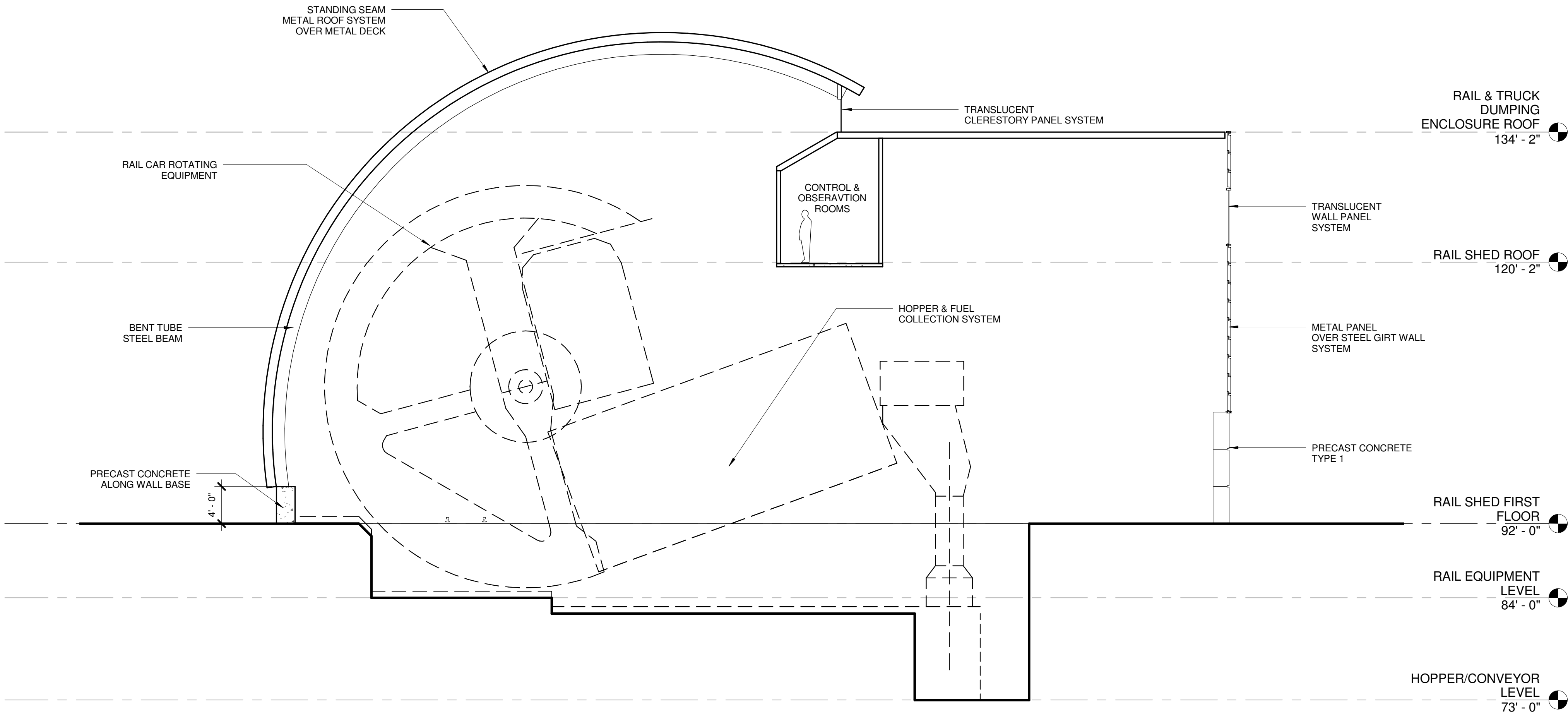
1 ROTARY DUMPER SECTION A307 1/8" = 1'-0"
