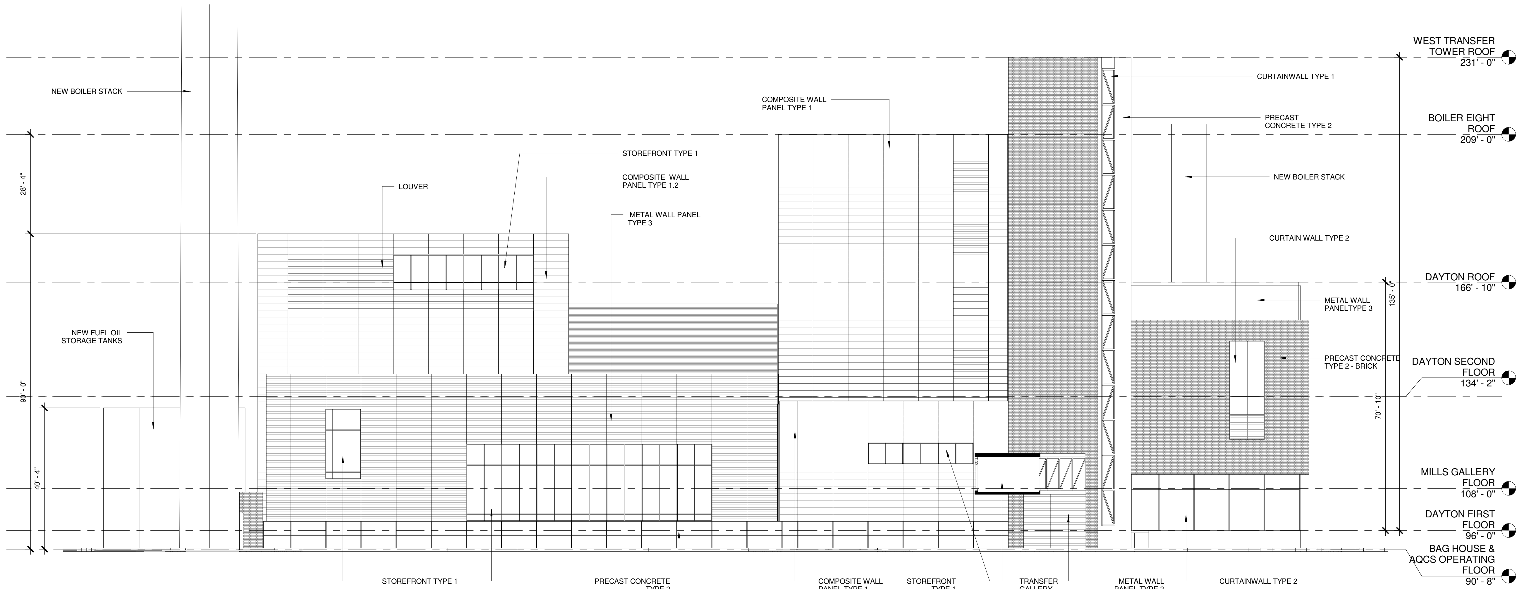
1 EAST ELEVATION - HEATING PLANT 1/16" = 1'-0"
