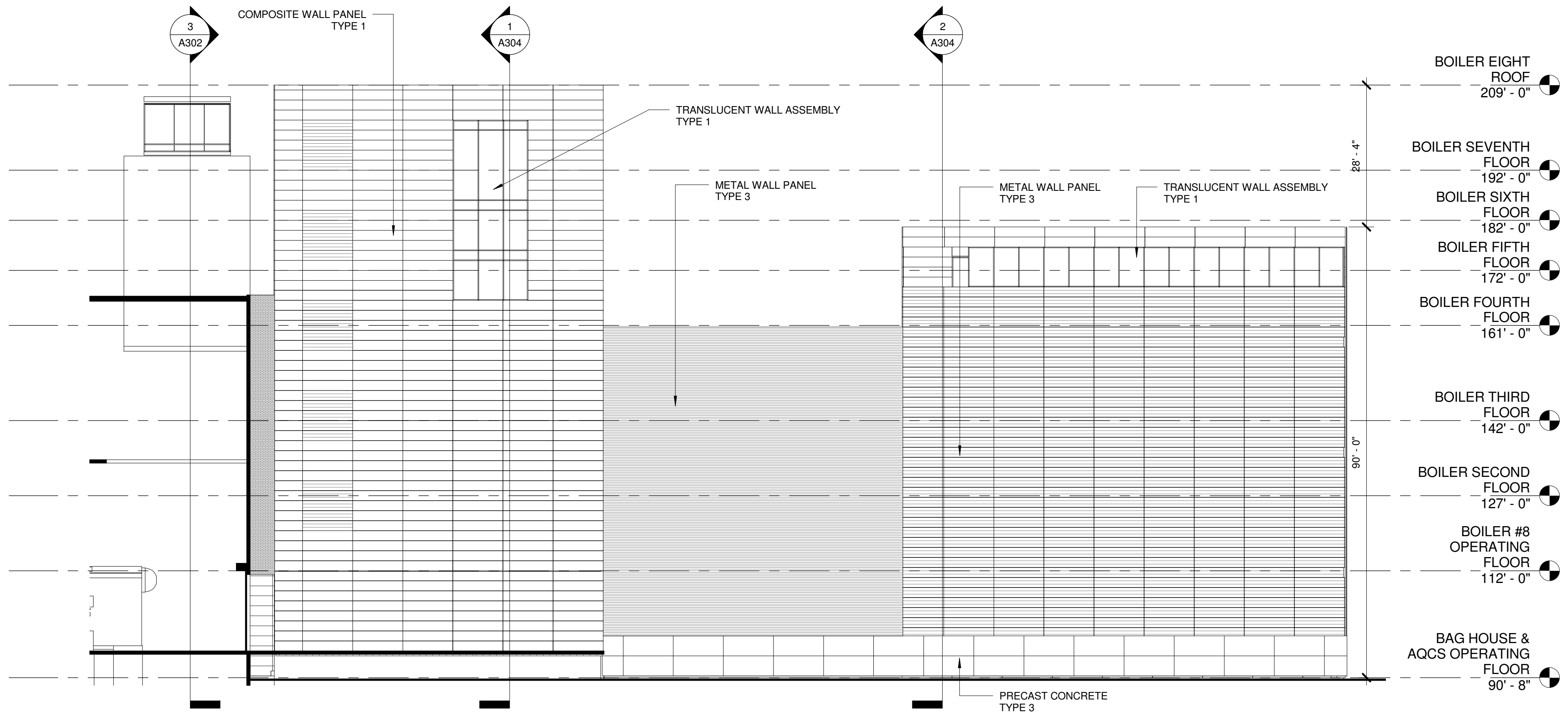
2 WEST ELEVATION - HEATING PLANT 1/16" = 1'-0"
