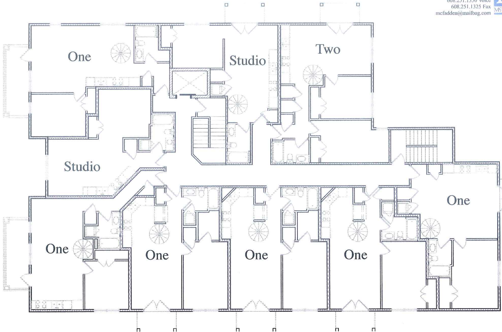
Proposed Third Floor Plan @ 1/12" = 1'-0" 119-25 North Butler Madison, Wisconsin May 7, 2007
