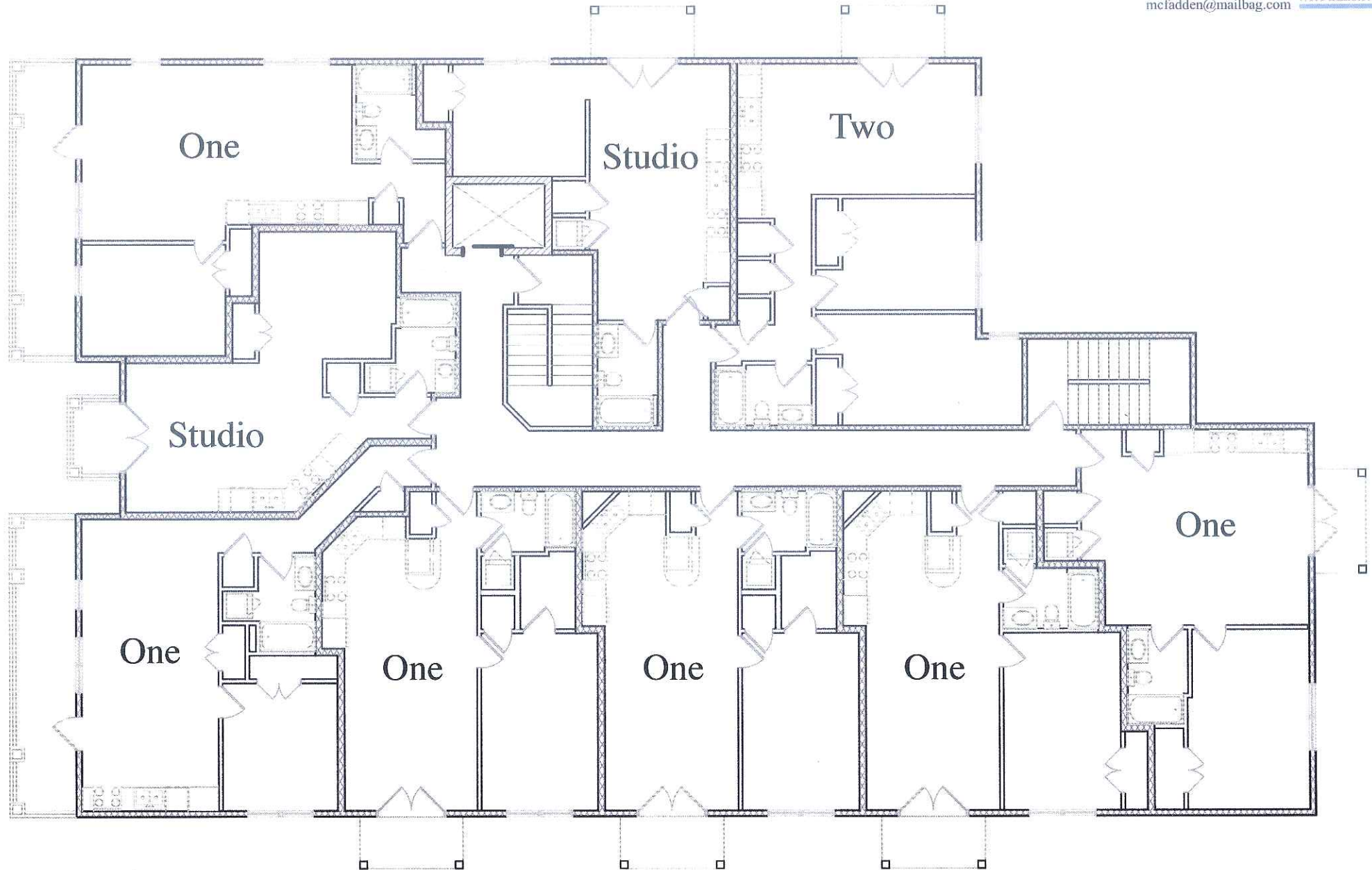
Proposed Second Floor Plan @ 1/12" = 1'-0" 119-25 North Butler Madison, Wisconsin May 7, 2007
