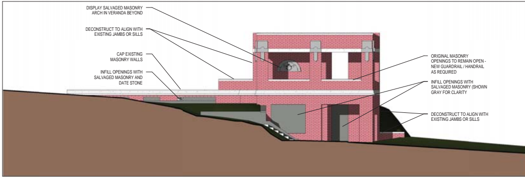
WEST ELEVATION
