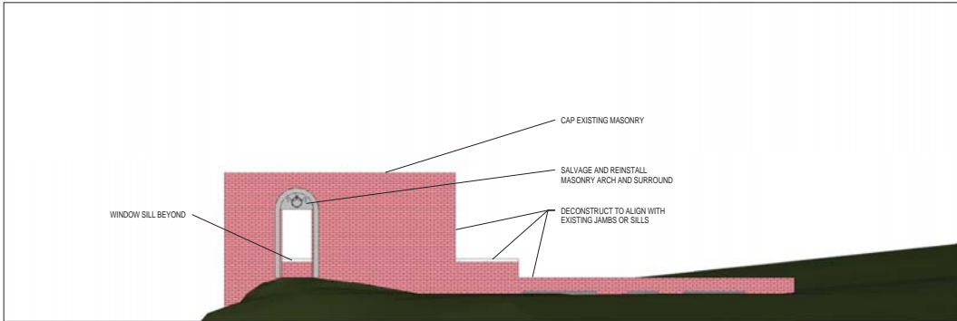
EAST ELEVATION
