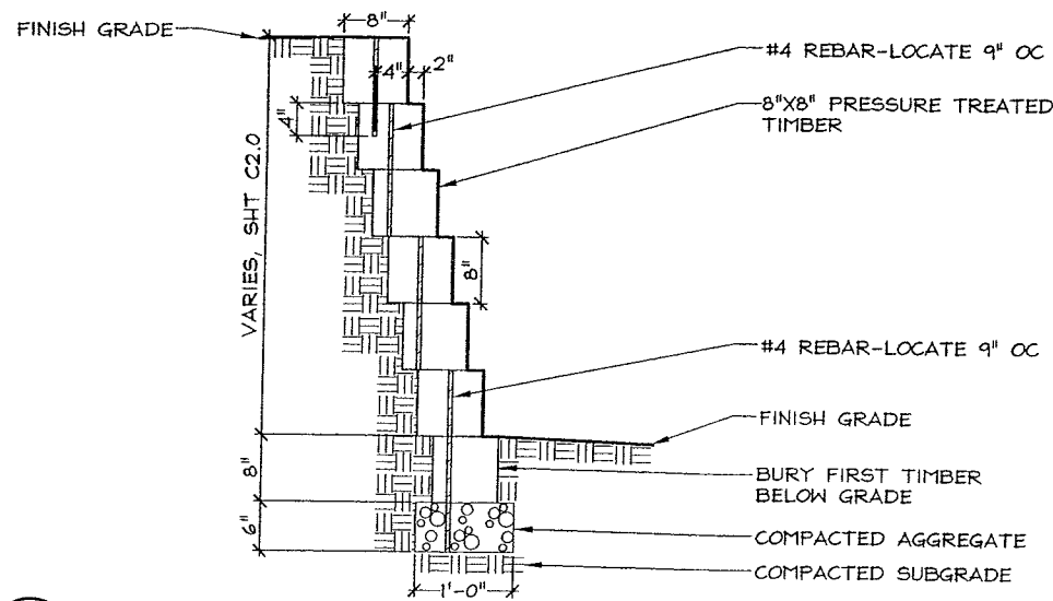
1 TIMBER RETAINING WALL C7.0 SCALE 1" = 1'-0"
