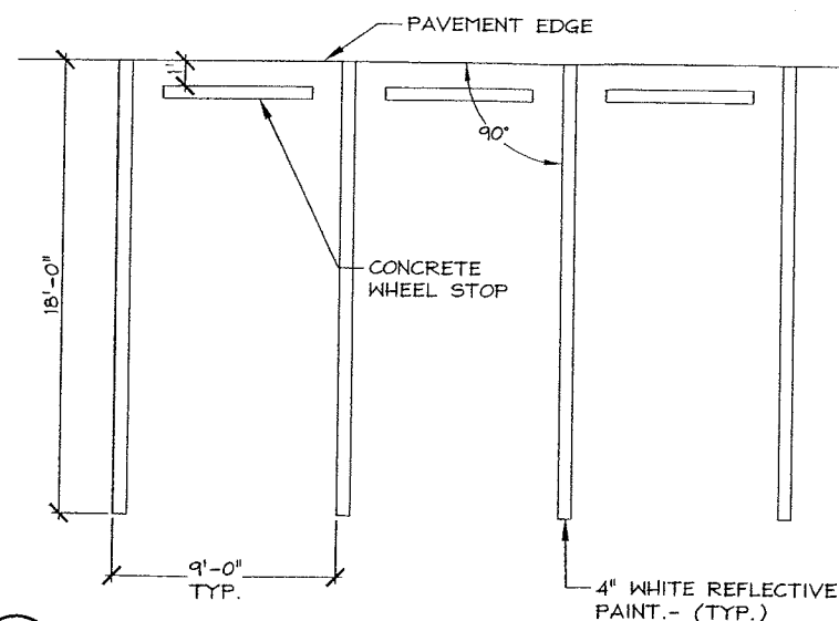
8 PAVEMENT MARKING C6.0 SCALE 1/4\"/>
