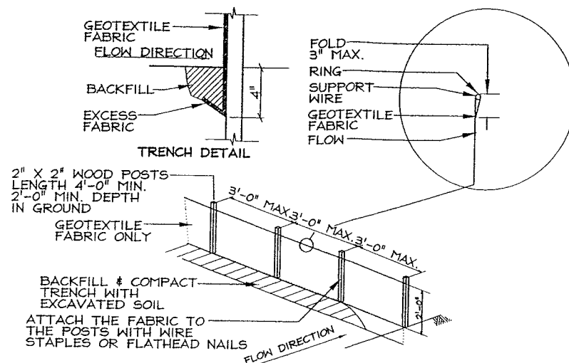
2 SILT FENCE DETAIL C6.0 NTS
