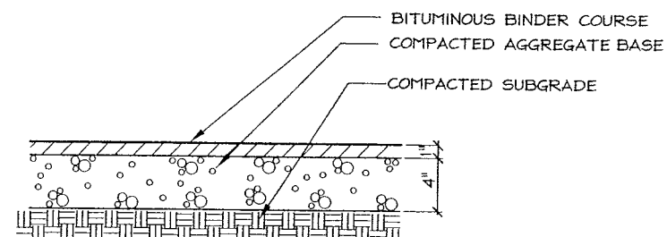
6 BITUMINOUS PAVEMENT BID ALTERNATE SECTION C6.0 SCALE 2\"/>
