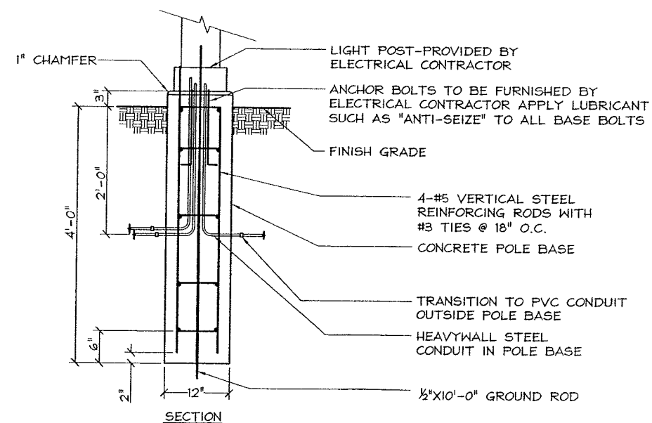
9 LIGHT BASE C6.0 SCALE 1\"/>
