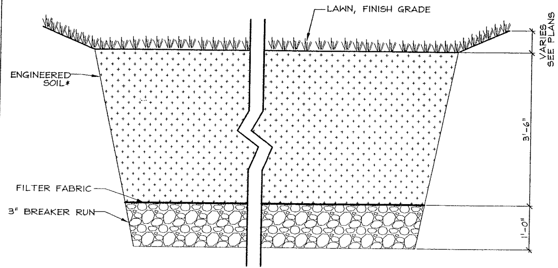
4 BIORETENTION DEVICE C7.0 SCALE 1" = 1'-0"
