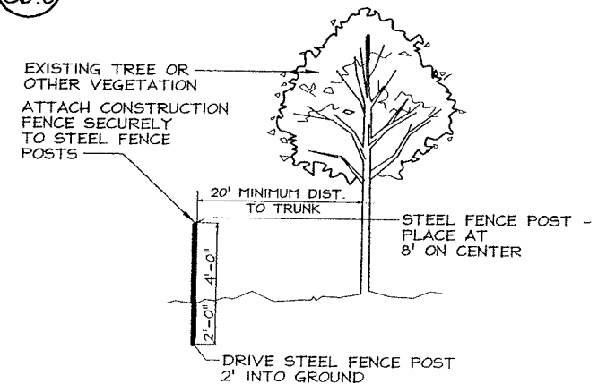
4 TREE PROTECTION DETAIL C6.0 NTS
