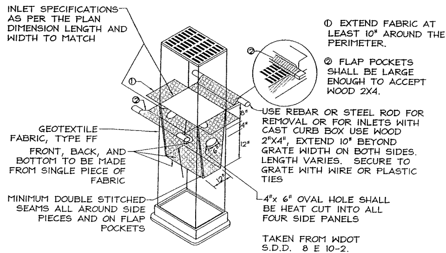
1 WISDOT INLET PROTECTION, TYPE D C6.0 NTS
