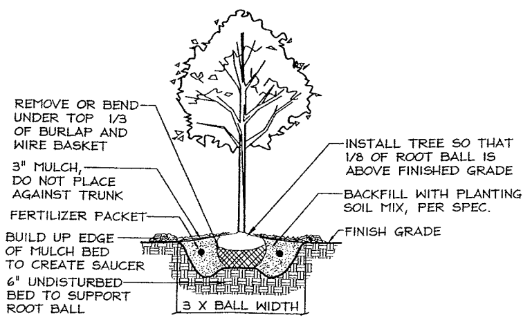
2 B&B TREE PLANTING DETAIL C7.0 NTS
