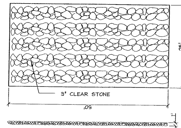
3 TRACK MAT DETAIL C6.0 SCALE 1/8\"/>
