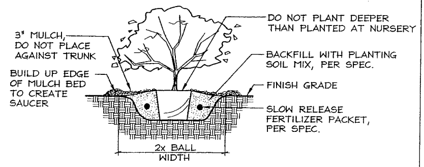
3 CONTAINER PLANTING DETAIL C7.0 NTS
