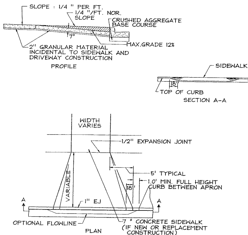
7 CLASS III DRIVE APRON C6.0 NTS
