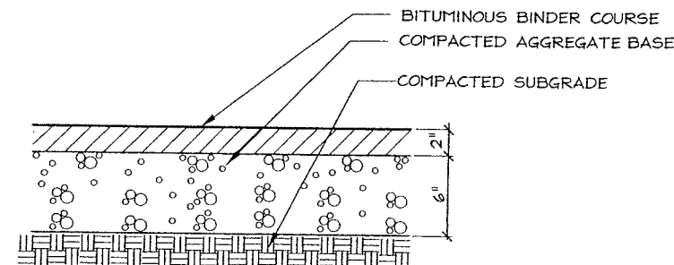
5 BITUMINOUS PAVEMENT SECTION C6.0 SCALE 2\"/>
