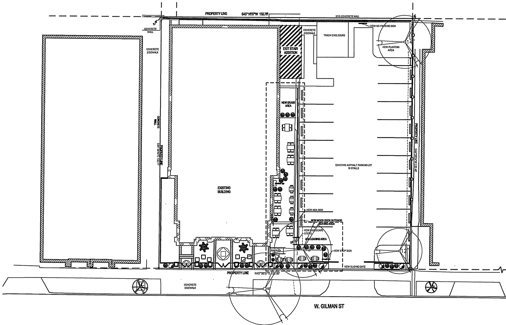
1 SITE PLAN 1" = 20'-0"
