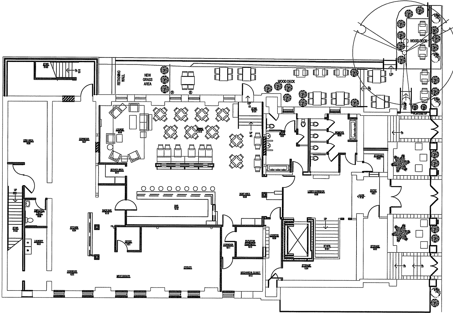
1 FIRST FLOOR PLAN & OUTDOOR SEATING AREA 3/32" = 1'-0"
