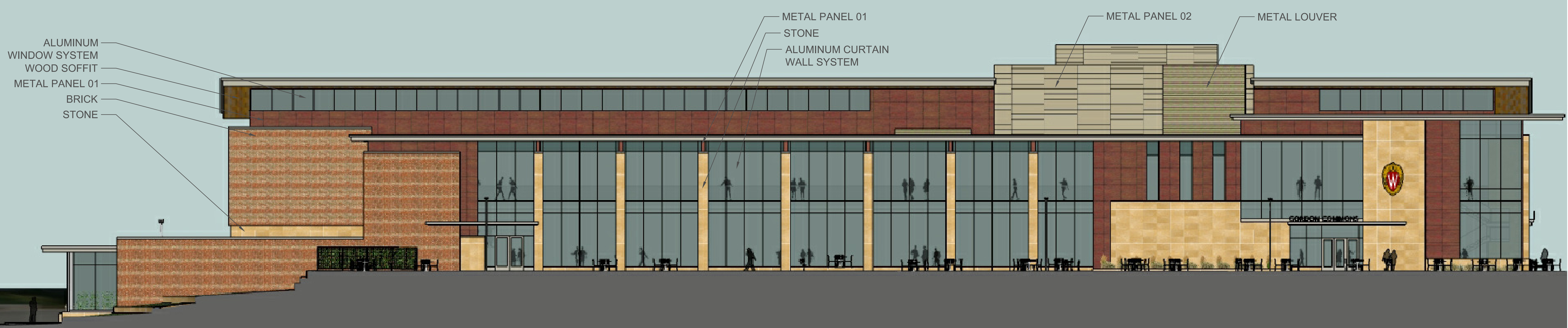
1 NORTH ELEVATION A201
