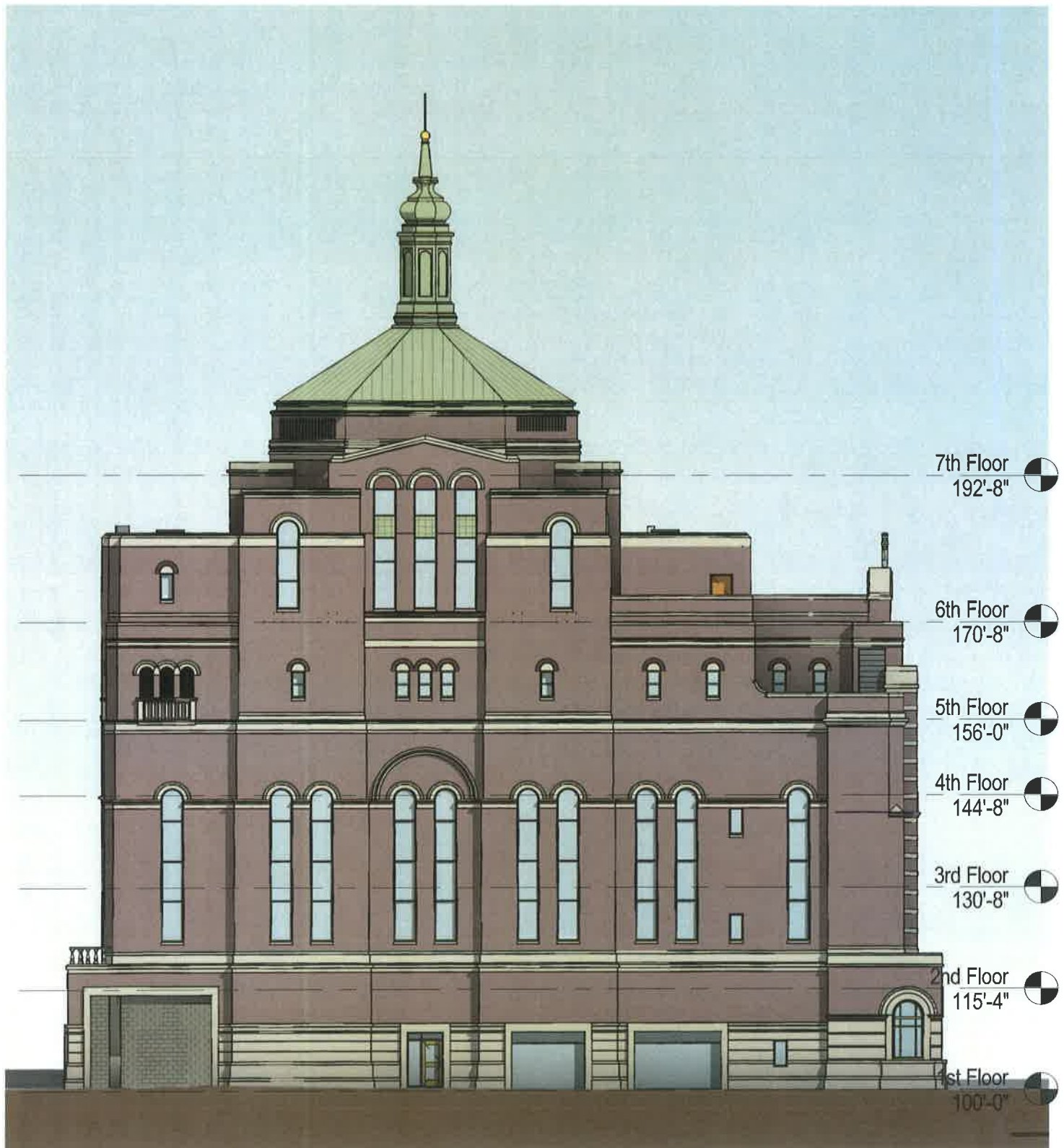
ELEVATION - EAST 1" = 20'-0"
