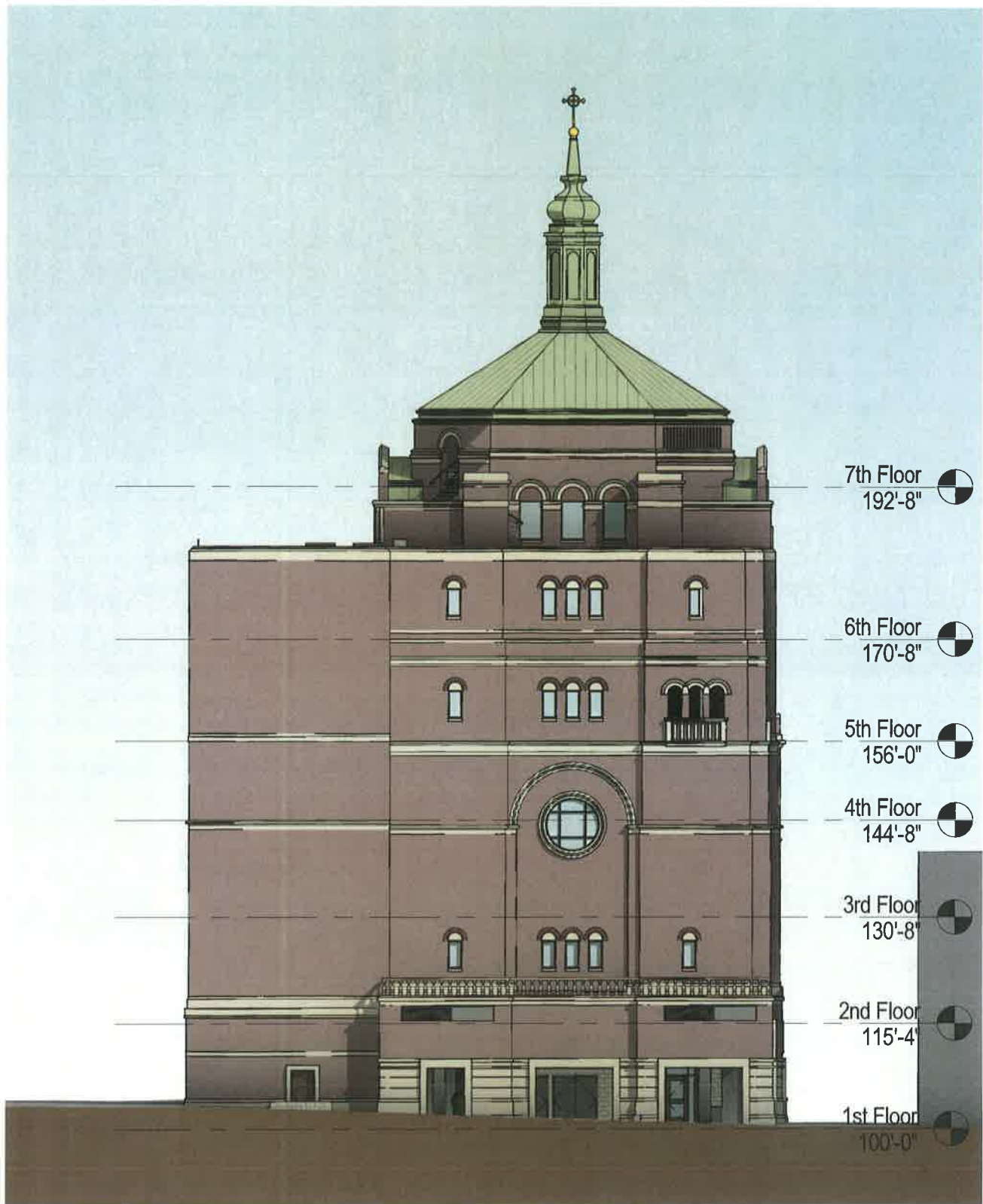
South Elevation
