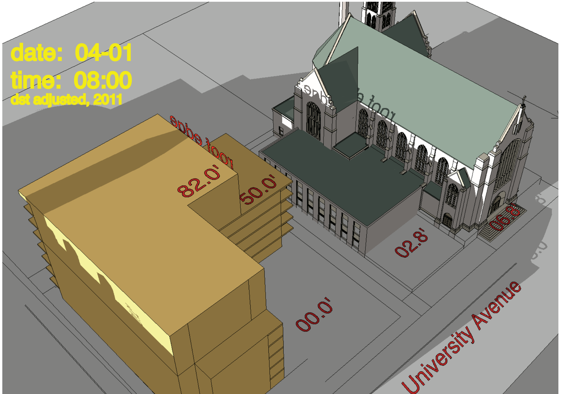
Luther Memorial Church Shading Study - Madison, WI 8 Story Option
